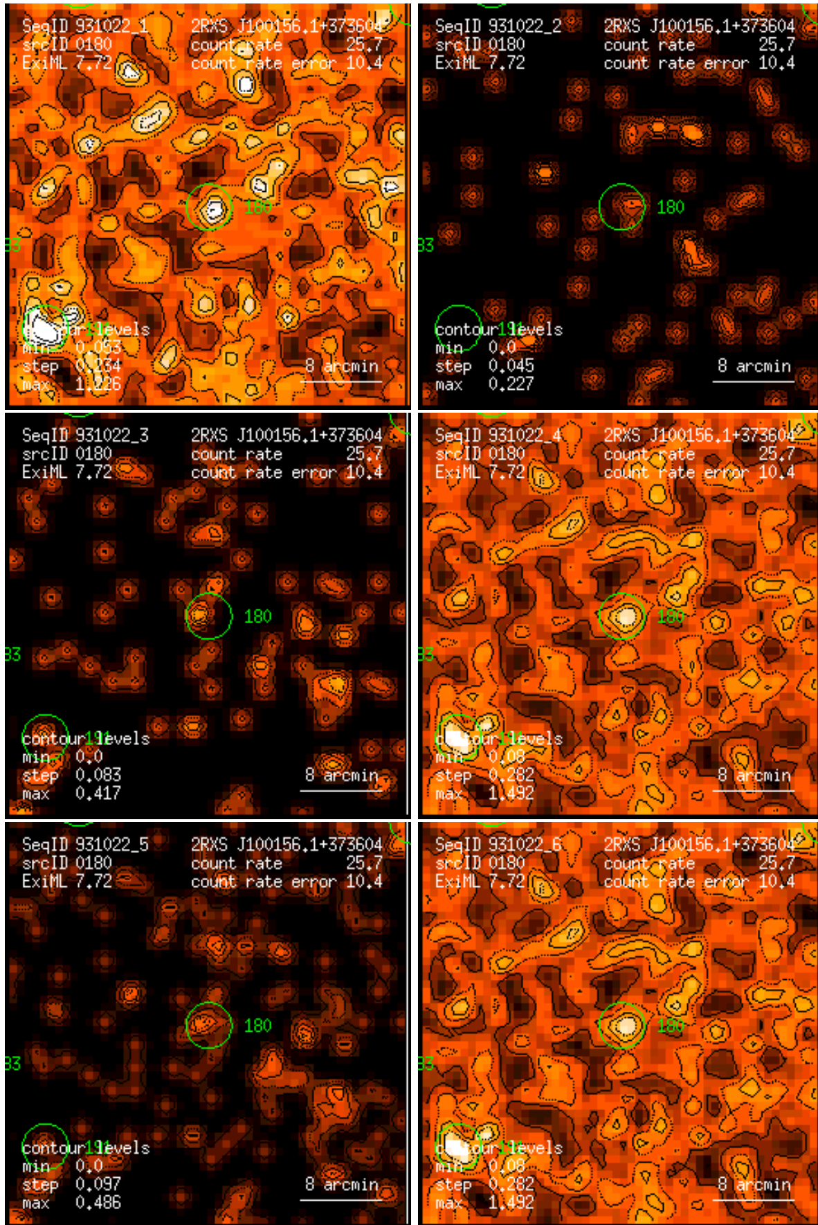
Figure 180: RASS 931022: detection 0180: band rate images, Gaussian filter: (1) PSPC channels 11 – 41, (2) 52 – 90, (3) 91 – 201, (4) 11 – 235, (5) 52 – 201, (6) 11 – 201. Broad band rates in counts/ks. Band rate contour levels in counts/ks/arcmin 2 .
