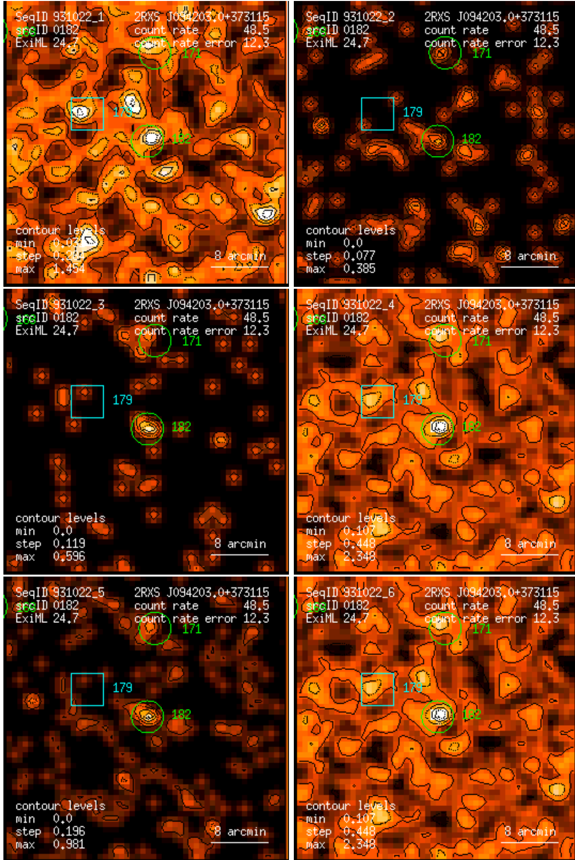
Figure 182: RASS 931022: detection 0182: band rate images, Gaussian filter: (1) PSPC channels 11 – 41, (2) 52 – 90, (3) 91 – 201, (4) 11 – 235, (5) 52 – 201, (6) 11 – 201. Broad band rates in counts/ks. Band rate contour levels in counts/ks/arcmin 2 .
