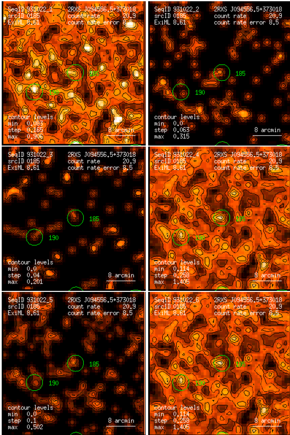
Figure 185: RASS 931022: detection 0185: band rate images, Gaussian filter: (1) PSPC channels 11 – 41, (2) 52 – 90, (3) 91 – 201, (4) 11 – 235, (5) 52 – 201, (6) 11 – 201. Broad band rates in counts/ks. Band rate contour levels in counts/ks/arcmin 2 .
