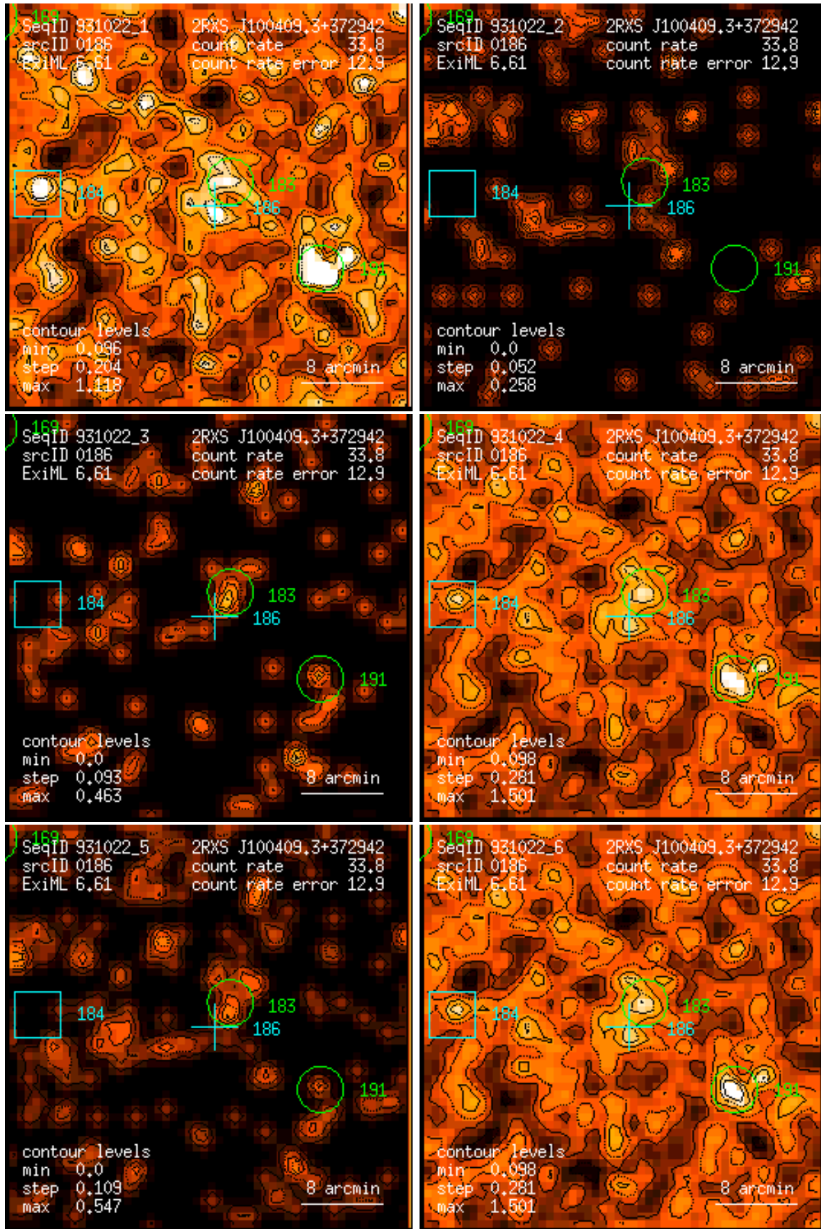
Figure 186: RASS 931022: detection 0186: band rate images, Gaussian filter: (1) PSPC channels 11 – 41, (2) 52 – 90, (3) 91 – 201, (4) 11 – 235, (5) 52 – 201, (6) 11 – 201. Broad band rates in counts/ks. Band rate contour levels in counts/ks/arcmin 2 .
