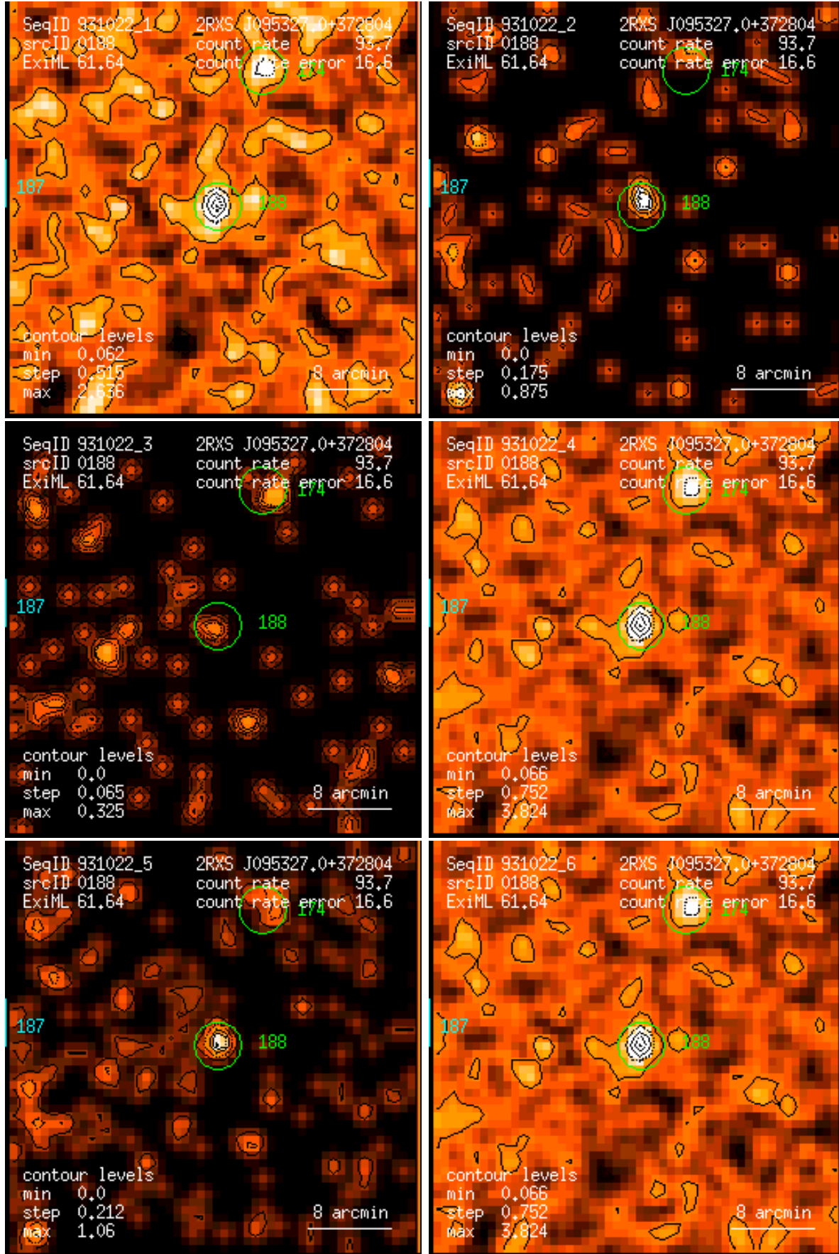
Figure 188: RASS 931022: detection 0188: band rate images, Gaussian filter: (1) PSPC channels 11 – 41, (2) 52 – 90, (3) 91 – 201, (4) 11 – 235, (5) 52 – 201, (6) 11 – 201. Broad band rates in counts/ks. Band rate contour levels in counts/ks/arcmin 2 .
