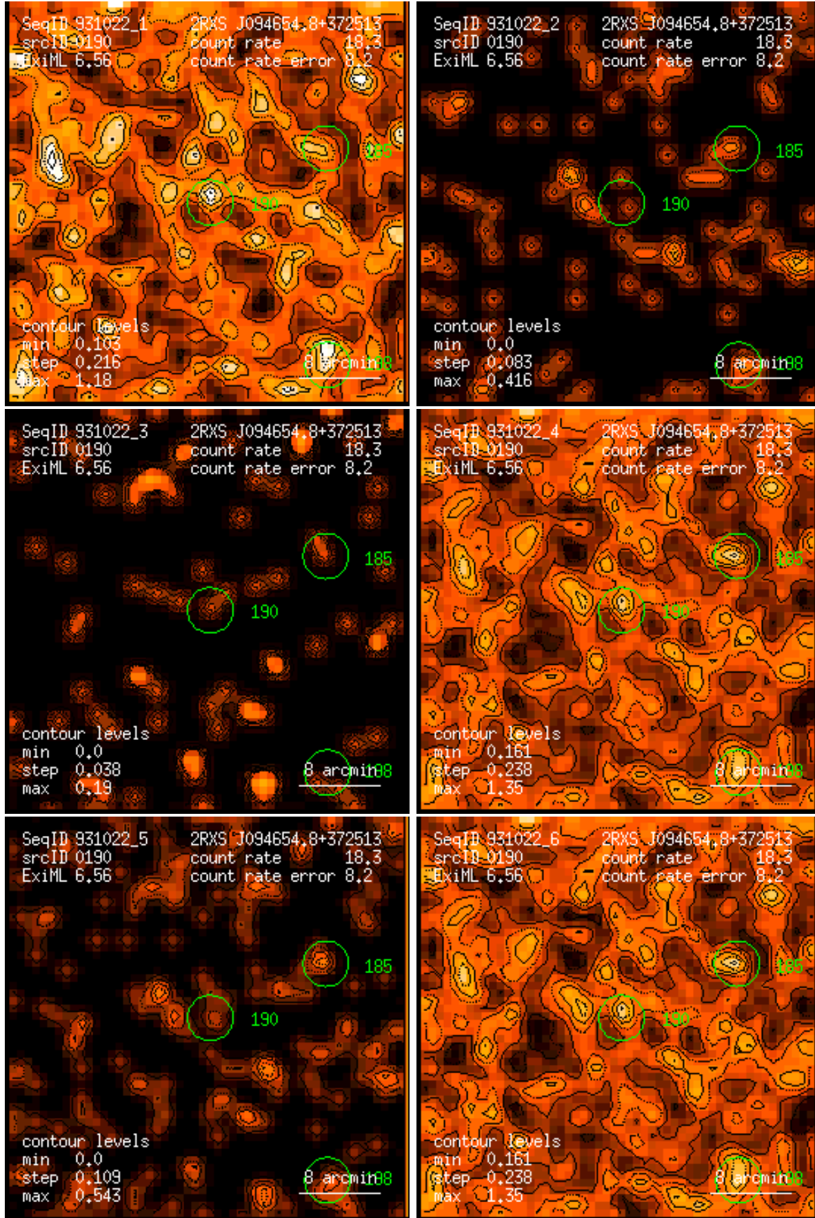
Figure 190: RASS 931022: detection 0190: band rate images, Gaussian filter: (1) PSPC channels 11 – 41, (2) 52 – 90, (3) 91 – 201, (4) 11 – 235, (5) 52 – 201, (6) 11 – 201. Broad band rates in counts/ks. Band rate contour levels in counts/ks/arcmin 2 .
