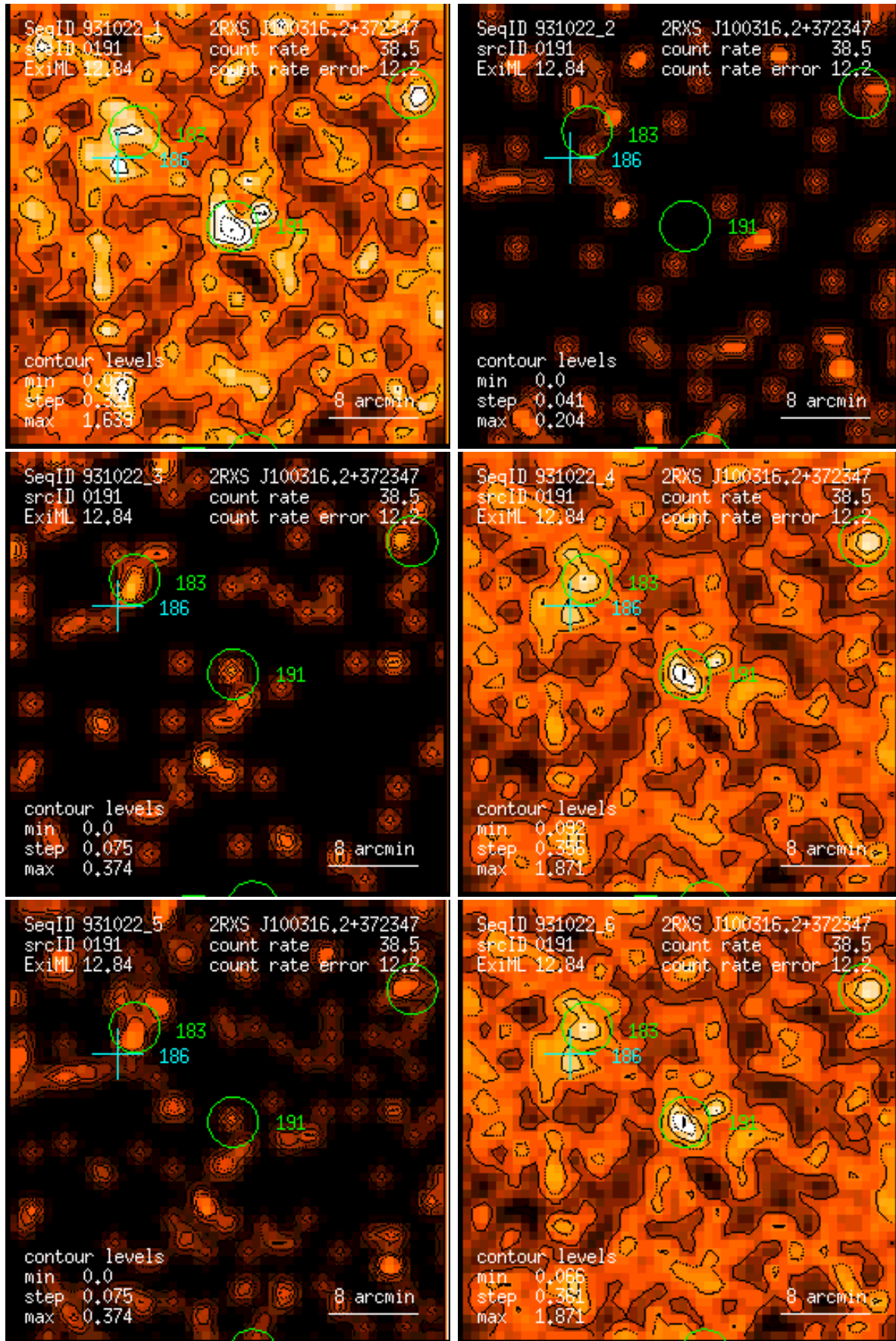
Figure 191: RASS 931022: detection 0191: band rate images, Gaussian filter: (1) PSPC channels 11 – 41, (2) 52 – 90, (3) 91 – 201, (4) 11 – 235, (5) 52 – 201, (6) 11 – 201. Broad band rates in counts/ks. Band rate contour levels in counts/ks/arcmin 2 .
