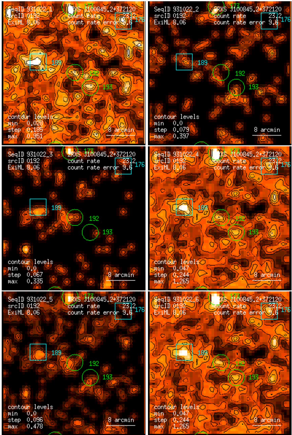
Figure 192: RASS 931022: detection 0192: band rate images, Gaussian filter: (1) PSPC channels 11 – 41, (2) 52 – 90, (3) 91 – 201, (4) 11 – 235, (5) 52 – 201, (6) 11 – 201. Broad band rates in counts/ks. Band rate contour levels in counts/ks/arcmin 2 .
