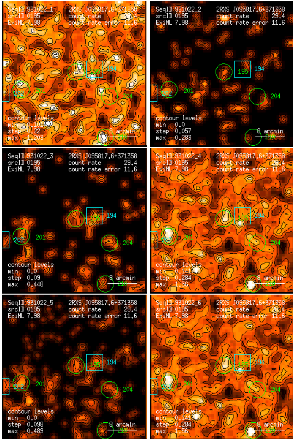
Figure 195: RASS 931022: detection 0195: band rate images, Gaussian filter: (1) PSPC channels 11 – 41, (2) 52 – 90, (3) 91 – 201, (4) 11 – 235, (5) 52 – 201, (6) 11 – 201. Broad band rates in counts/ks. Band rate contour levels in counts/ks/arcmin 2 .
