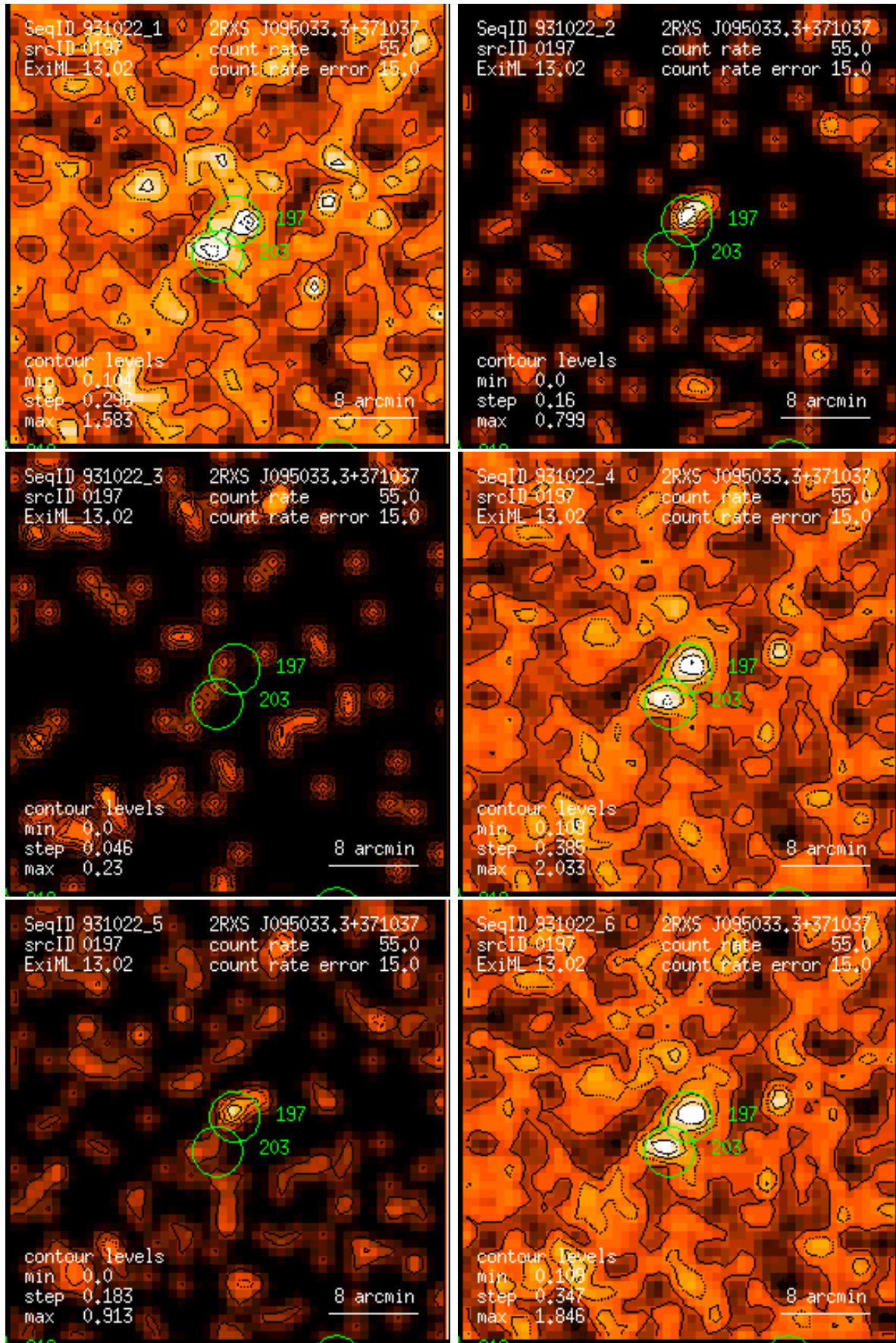
Figure 197: RASS 931022: detection 0197: band rate images, Gaussian filter: (1) PSPC channels 11 – 41, (2) 52 – 90, (3) 91 – 201, (4) 11 – 235, (5) 52 – 201, (6) 11 – 201. Broad band rates in counts/ks. Band rate contour levels in counts/ks/arcmin 2 .
