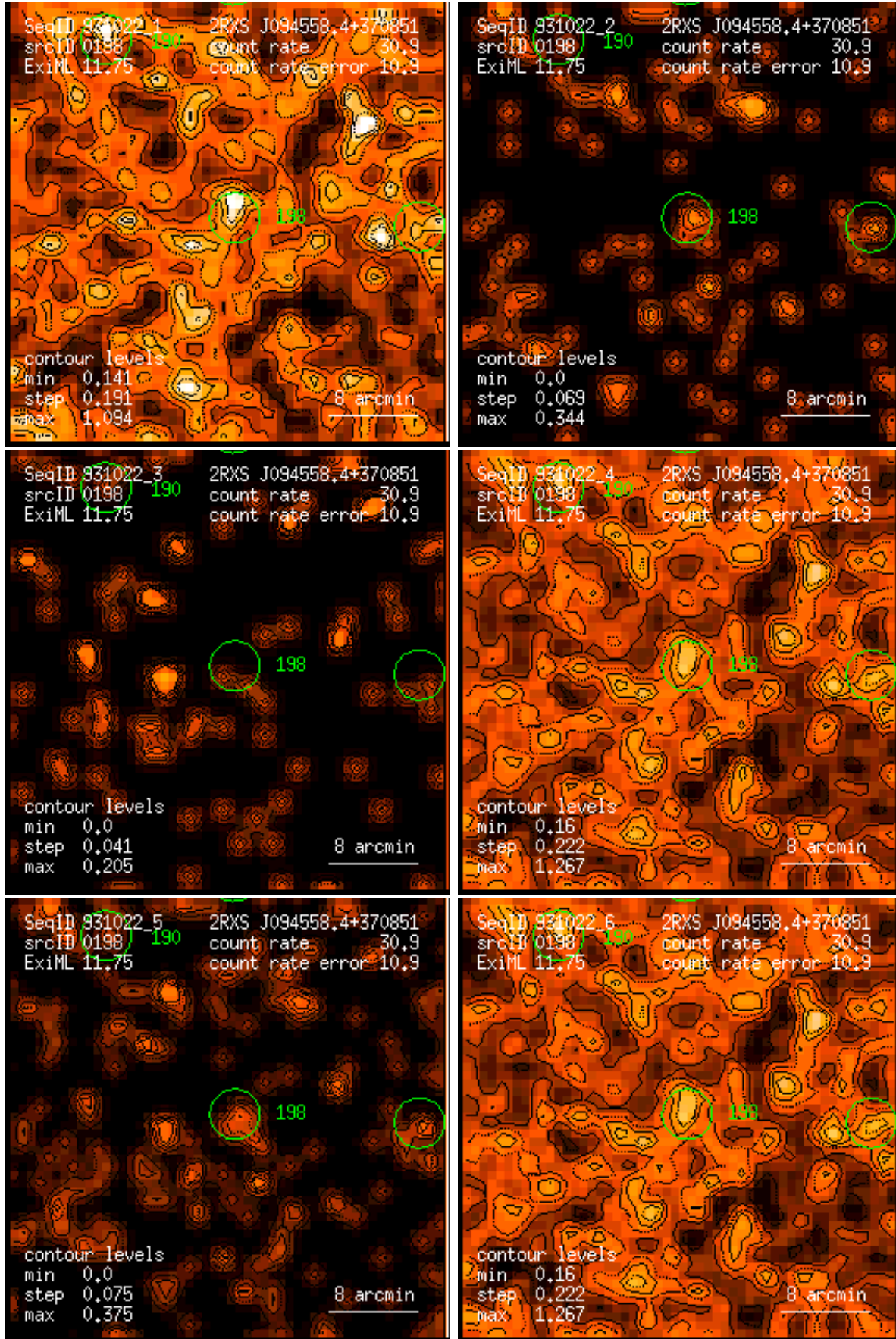
Figure 198: RASS 931022: detection 0198: band rate images, Gaussian filter: (1) PSPC channels 11 – 41, (2) 52 – 90, (3) 91 – 201, (4) 11 – 235, (5) 52 – 201, (6) 11 – 201. Broad band rates in counts/ks. Band rate contour levels in counts/ks/arcmin 2 .
