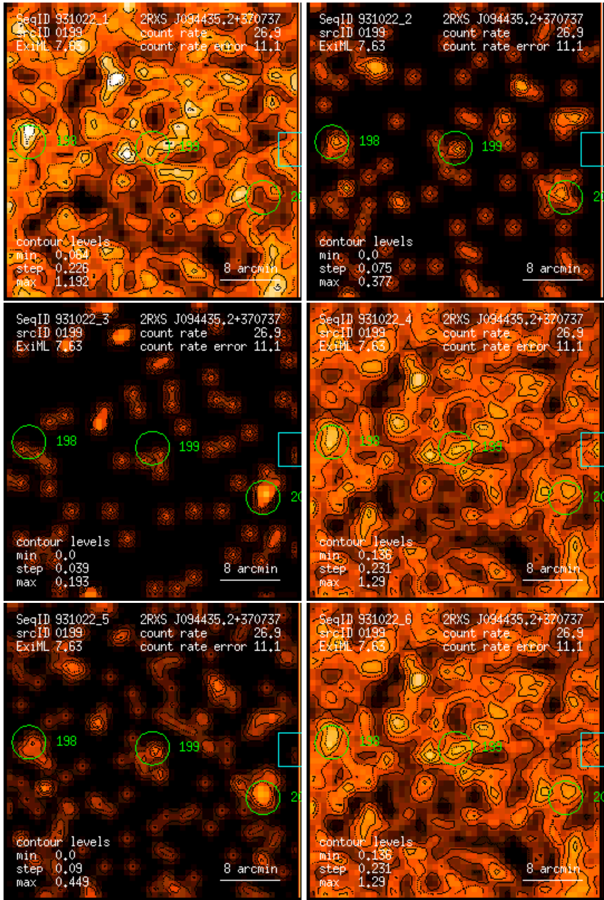
Figure 199: RASS 931022: detection 0199: band rate images, Gaussian filter: (1) PSPC channels 11 – 41, (2) 52 – 90, (3) 91 – 201, (4) 11 – 235, (5) 52 – 201, (6) 11 – 201. Broad band rates in counts/ks. Band rate contour levels in counts/ks/arcmin 2 .
