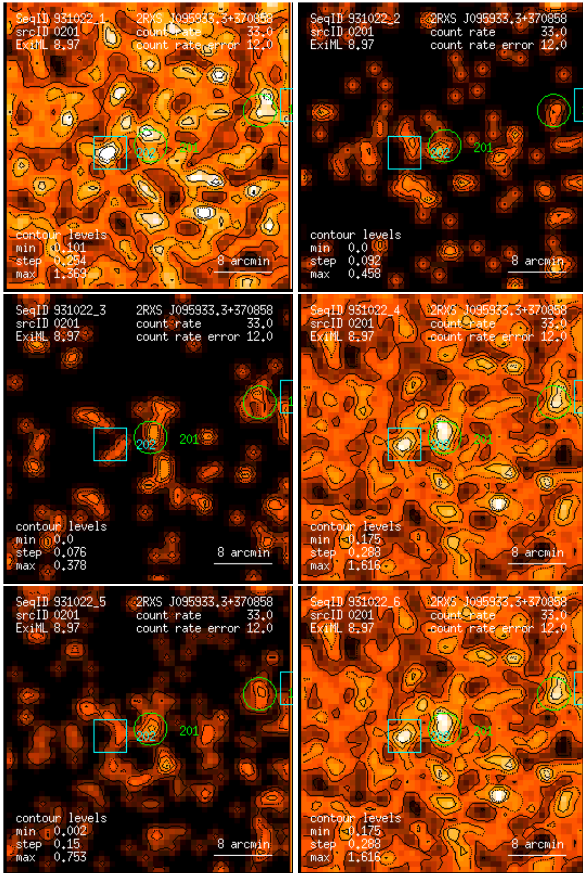
Figure 201: RASS 931022: detection 0201: band rate images, Gaussian filter: (1) PSPC channels 11 – 41, (2) 52 – 90, (3) 91 – 201, (4) 11 – 235, (5) 52 – 201, (6) 11 – 201. Broad band rates in counts/ks. Band rate contour levels in counts/ks/arcmin 2 .
