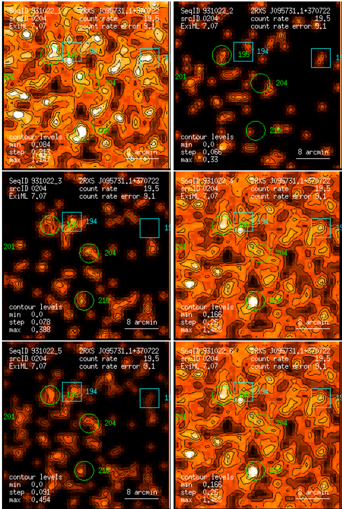
Figure 204: RASS 931022: detection 0204: band rate images, Gaussian filter: (1) PSPC channels 11 – 41, (2) 52 – 90, (3) 91 – 201, (4) 11 – 235, (5) 52 – 201, (6) 11 – 201. Broad band rates in counts/ks. Band rate contour levels in counts/ks/arcmin 2 .
