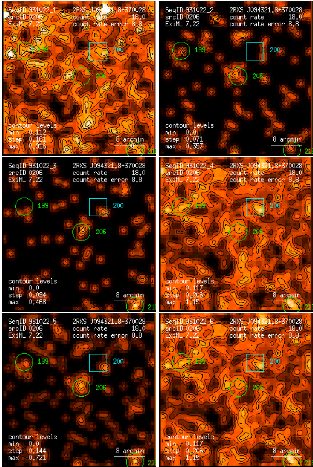
Figure 206: RASS 931022: detection 0206: band rate images, Gaussian filter: (1) PSPC channels 11 – 41, (2) 52 – 90, (3) 91 – 201, (4) 11 – 235, (5) 52 – 201, (6) 11 – 201. Broad band rates in counts/ks. Band rate contour levels in counts/ks/arcmin 2 .
