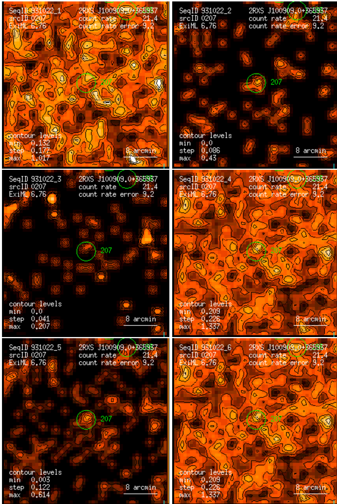
Figure 207: RASS 931022: detection 0207: band rate images, Gaussian filter: (1) PSPC channels 11 – 41, (2) 52 – 90, (3) 91 – 201, (4) 11 – 235, (5) 52 – 201, (6) 11 – 201. Broad band rates in counts/ks. Band rate contour levels in counts/ks/arcmin 2 .
