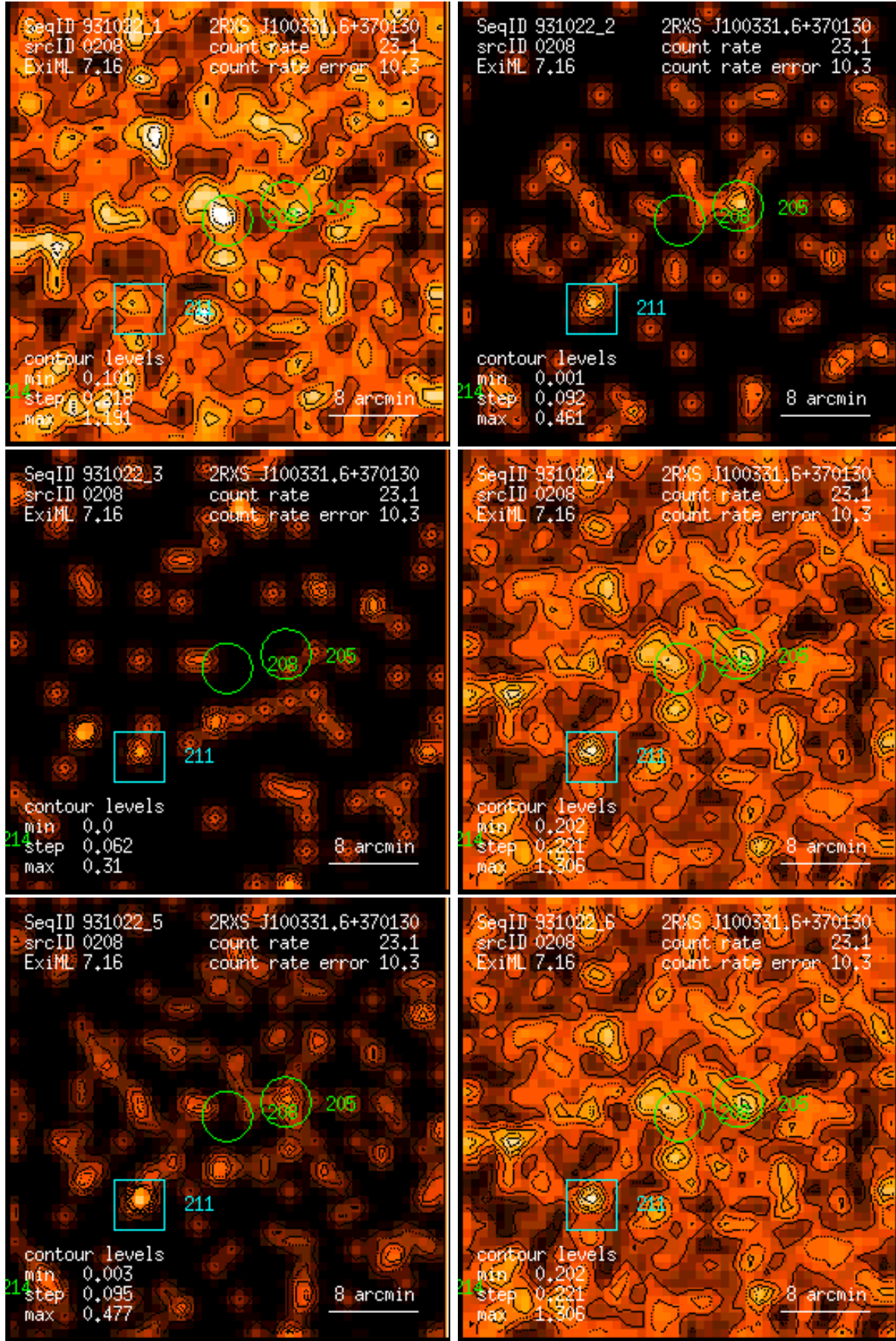
Figure 208: RASS 931022: detection 0208: band rate images, Gaussian filter: (1) PSPC channels 11 – 41, (2) 52 – 90, (3) 91 – 201, (4) 11 – 235, (5) 52 – 201, (6) 11 – 201. Broad band rates in counts/ks. Band rate contour levels in counts/ks/arcmin 2 .
