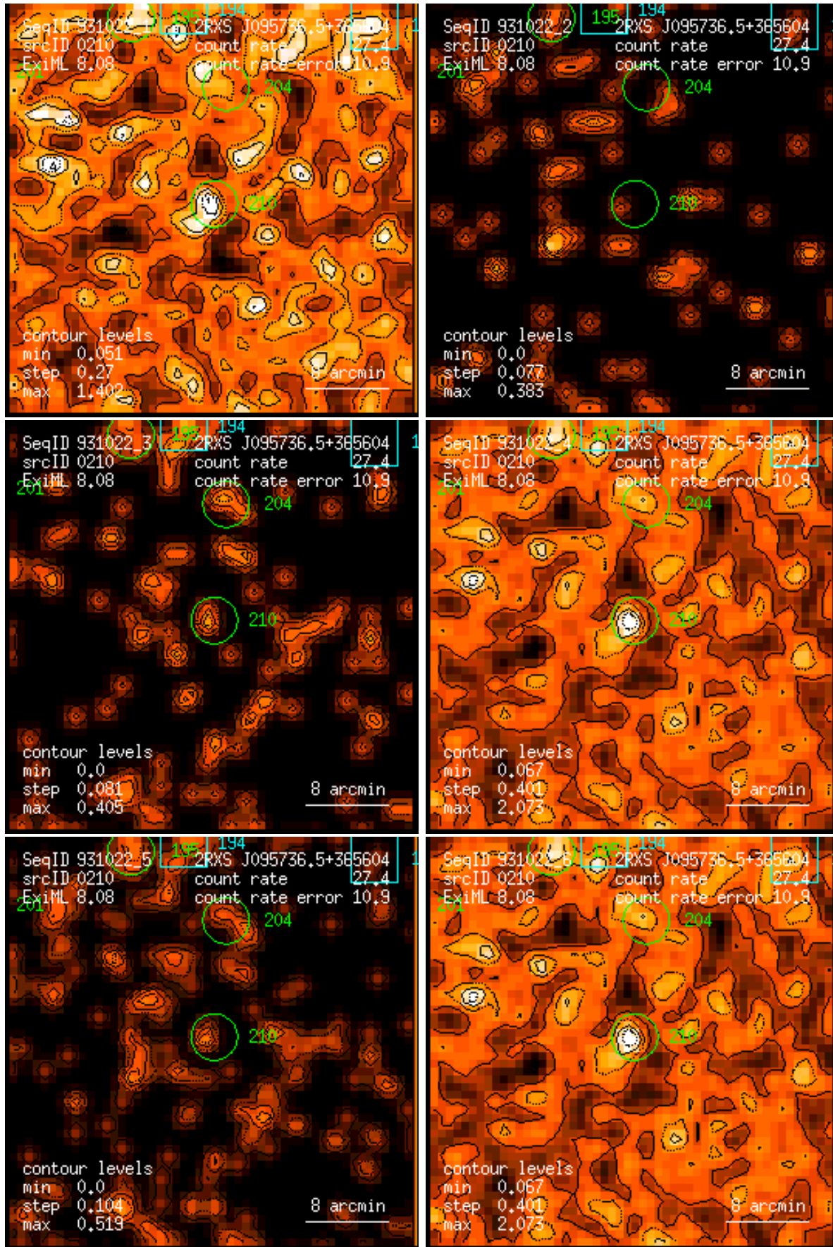
Figure 210: RASS 931022: detection 0210: band rate images, Gaussian filter: (1) PSPC channels 11 – 41, (2) 52 – 90, (3) 91 – 201, (4) 11 – 235, (5) 52 – 201, (6) 11 – 201. Broad band rates in counts/ks. Band rate contour levels in counts/ks/arcmin 2 .
