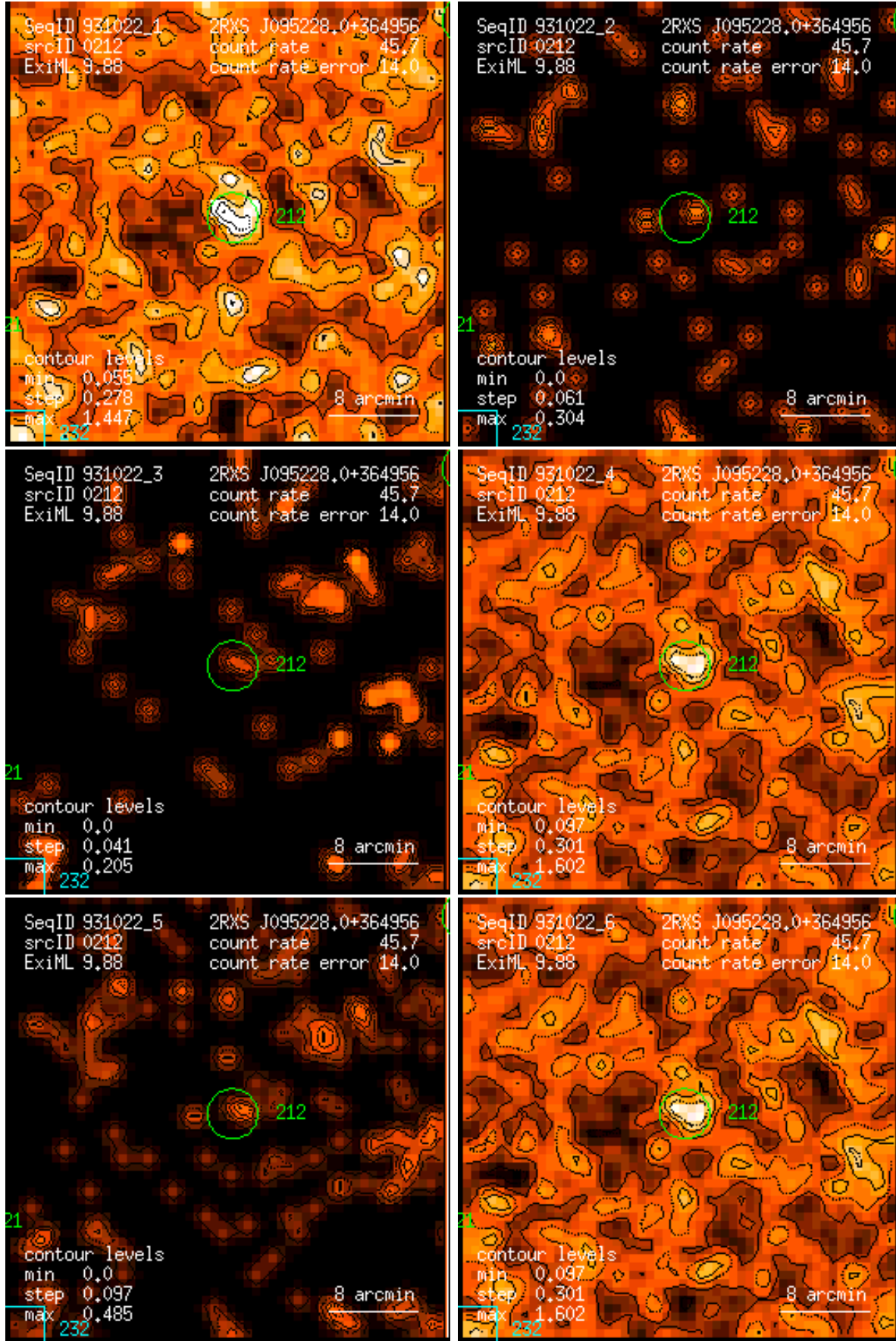
Figure 212: RASS 931022: detection 0212: band rate images, Gaussian filter: (1) PSPC channels 11 – 41, (2) 52 – 90, (3) 91 – 201, (4) 11 – 235, (5) 52 – 201, (6) 11 – 201. Broad band rates in counts/ks. Band rate contour levels in counts/ks/arcmin 2 .
