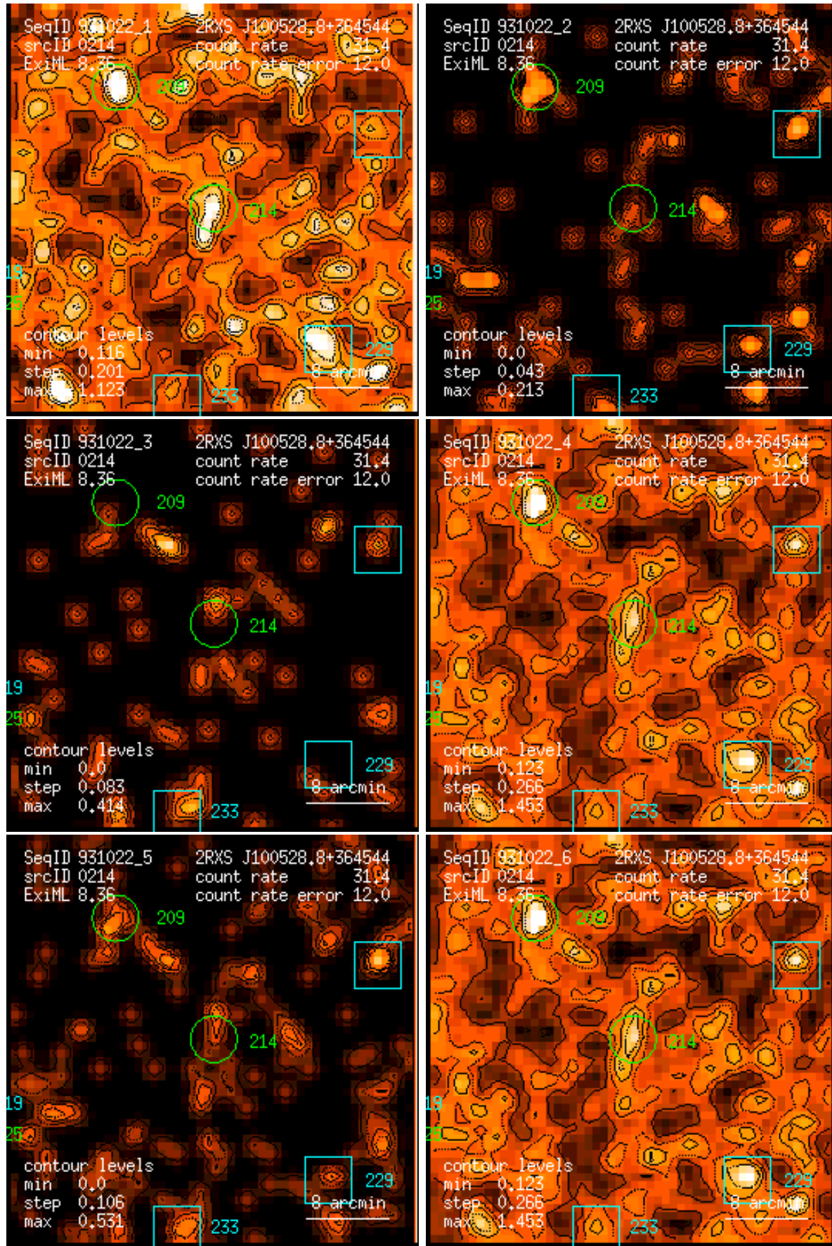
Figure 214: RASS 931022: detection 0214: band rate images, Gaussian filter: (1) PSPC channels 11 – 41, (2) 52 – 90, (3) 91 – 201, (4) 11 – 235, (5) 52 – 201, (6) 11 – 201. Broad band rates in counts/ks. Band rate contour levels in counts/ks/arcmin 2 .
