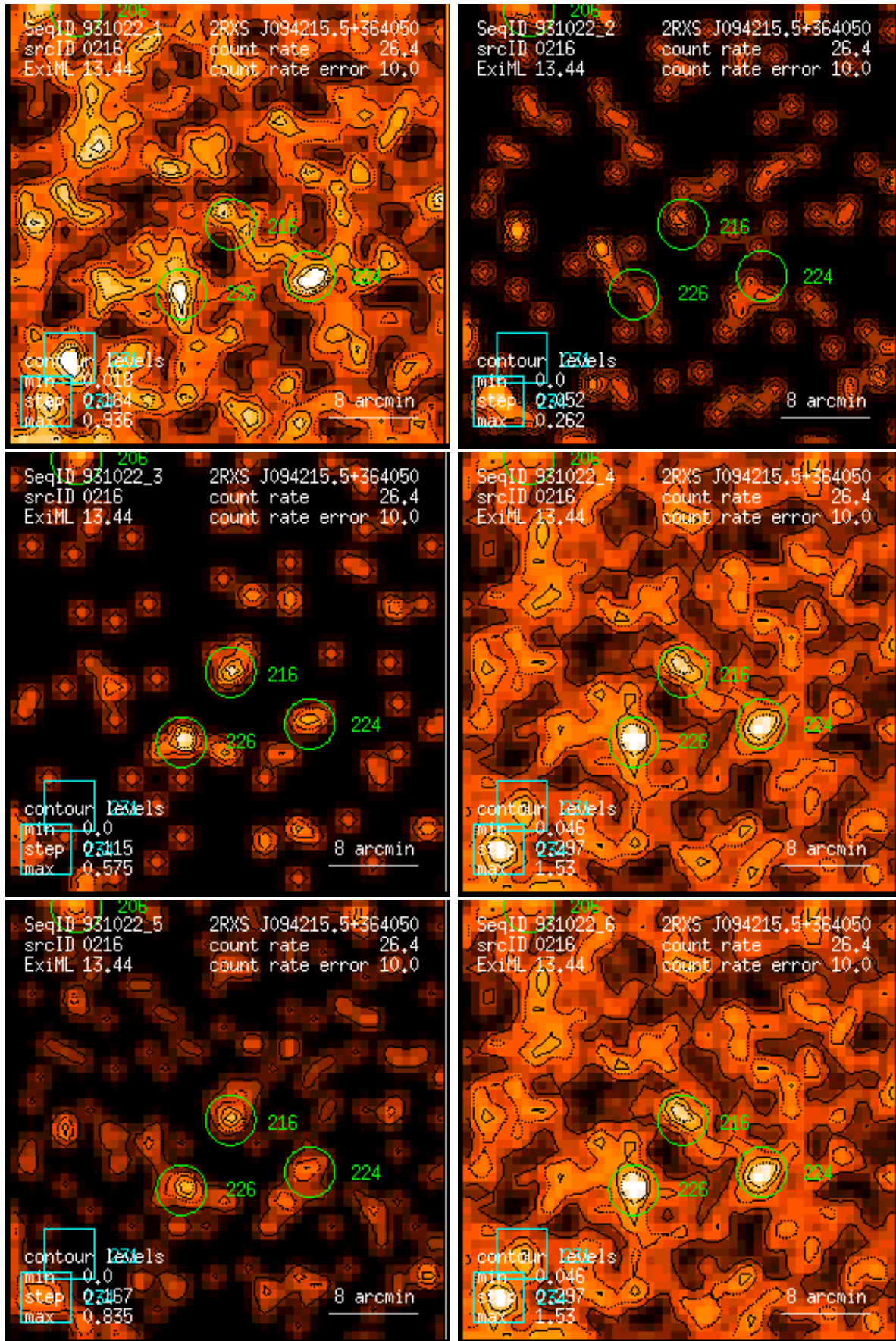
Figure 216: RASS 931022: detection 0216: band rate images, Gaussian filter: (1) PSPC channels 11 – 41, (2) 52 – 90, (3) 91 – 201, (4) 11 – 235, (5) 52 – 201, (6) 11 – 201. Broad band rates in counts/ks. Band rate contour levels in counts/ks/arcmin 2 .
