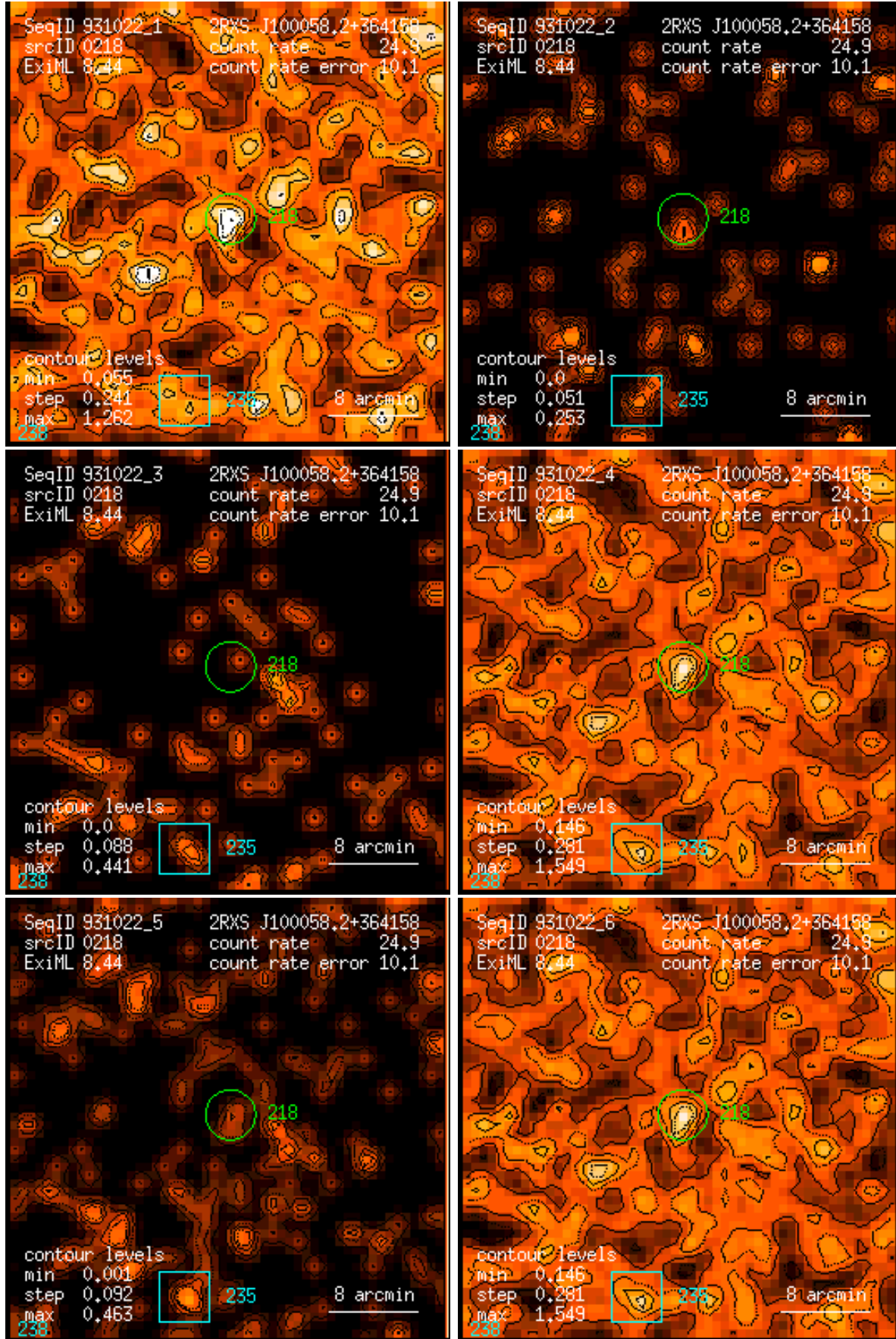
Figure 218: RASS 931022: detection 0218: band rate images, Gaussian filter: (1) PSPC channels 11 – 41, (2) 52 – 90, (3) 91 – 201, (4) 11 – 235, (5) 52 – 201, (6) 11 – 201. Broad band rates in counts/ks. Band rate contour levels in counts/ks/arcmin 2 .
