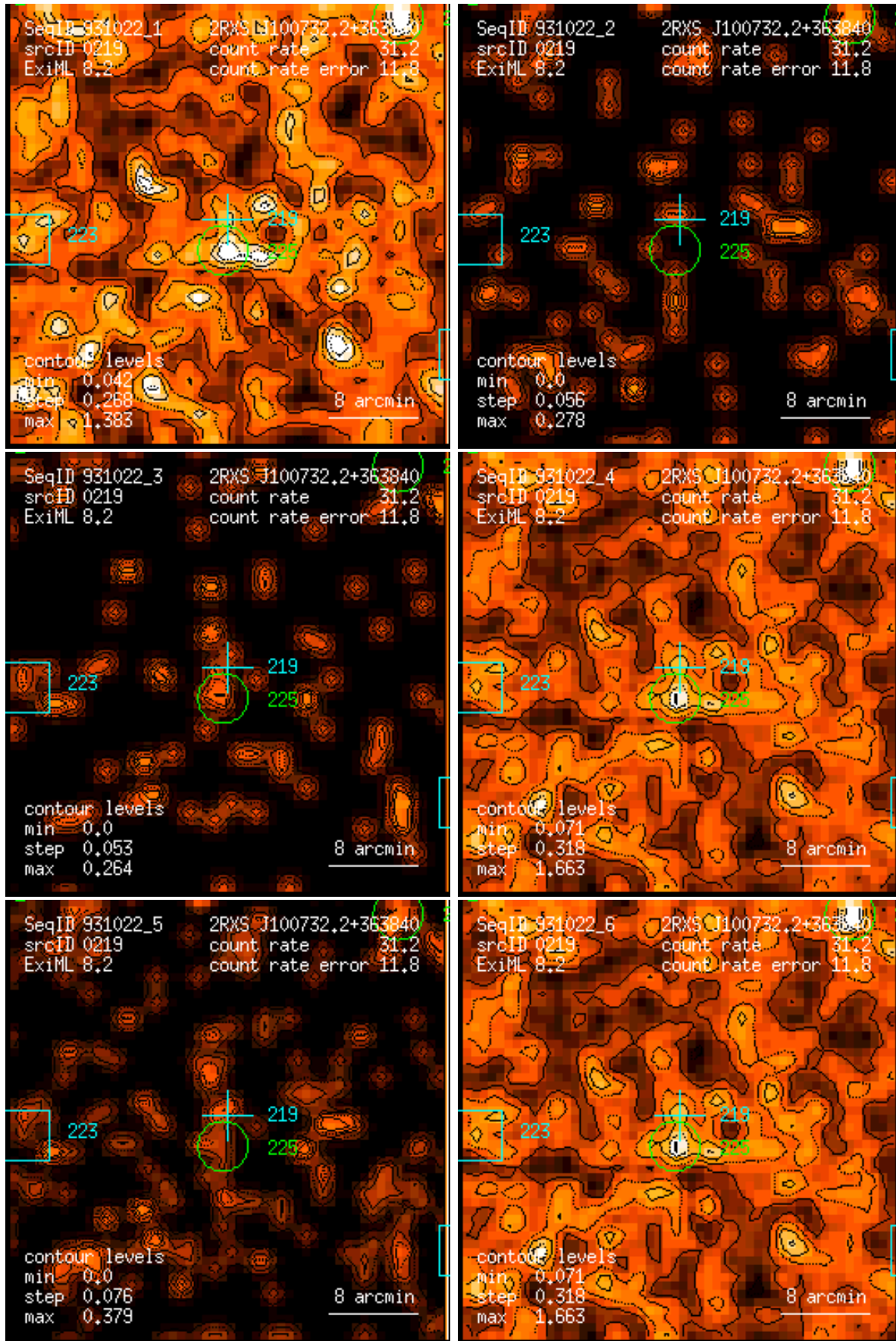
Figure 219: RASS 931022: detection 0219: band rate images, Gaussian filter: (1) PSPC channels 11 – 41, (2) 52 – 90, (3) 91 – 201, (4) 11 – 235, (5) 52 – 201, (6) 11 – 201. Broad band rates in counts/ks. Band rate contour levels in counts/ks/arcmin 2 .
