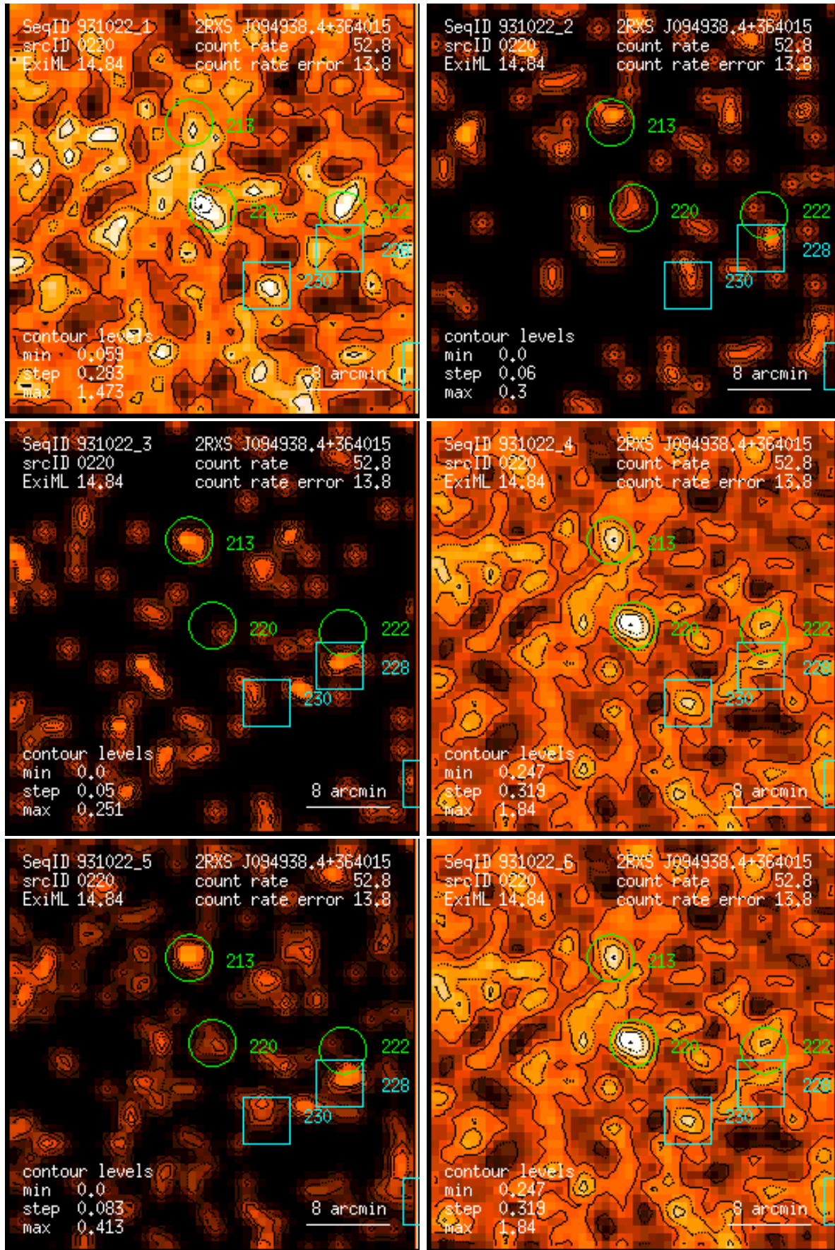
Figure 220: RASS 931022: detection 0220: band rate images, Gaussian filter: (1) PSPC channels 11 – 41, (2) 52 – 90, (3) 91 – 201, (4) 11 – 235, (5) 52 – 201, (6) 11 – 201. Broad band rates in counts/ks. Band rate contour levels in counts/ks/arcmin 2 .
