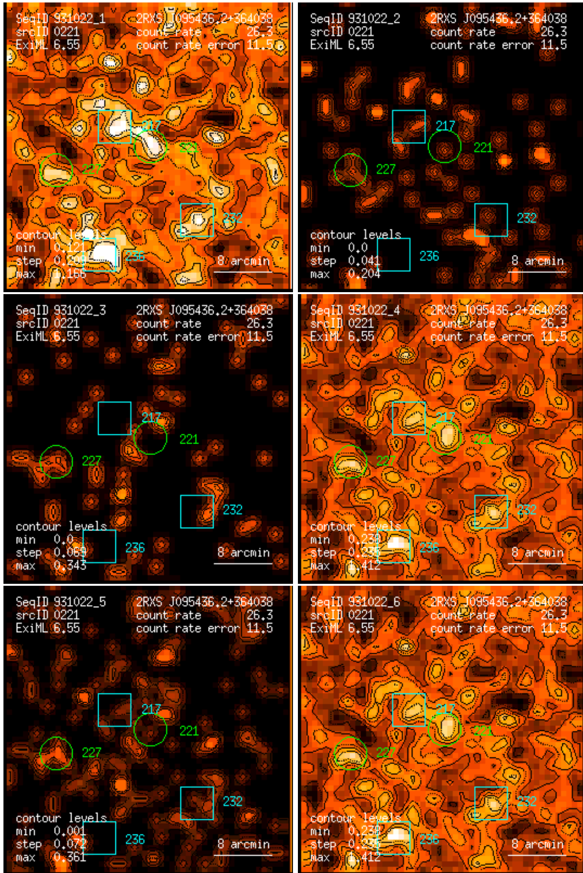
Figure 221: RASS 931022: detection 0221: band rate images, Gaussian filter: (1) PSPC channels 11 – 41, (2) 52 – 90, (3) 91 – 201, (4) 11 – 235, (5) 52 – 201, (6) 11 – 201. Broad band rates in counts/ks. Band rate contour levels in counts/ks/arcmin 2 .
