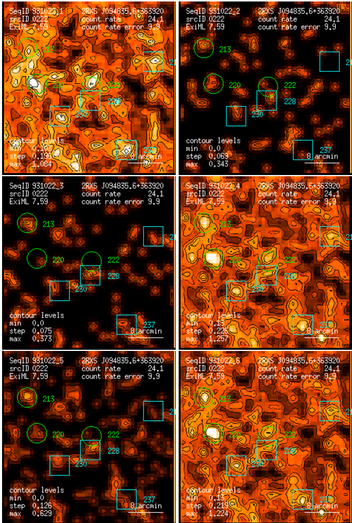
Figure 222: RASS 931022: detection 0222: band rate images, Gaussian filter: (1) PSPC channels 11 – 41, (2) 52 – 90, (3) 91 – 201, (4) 11 – 235, (5) 52 – 201, (6) 11 – 201. Broad band rates in counts/ks. Band rate contour levels in counts/ks/arcmin 2 .
