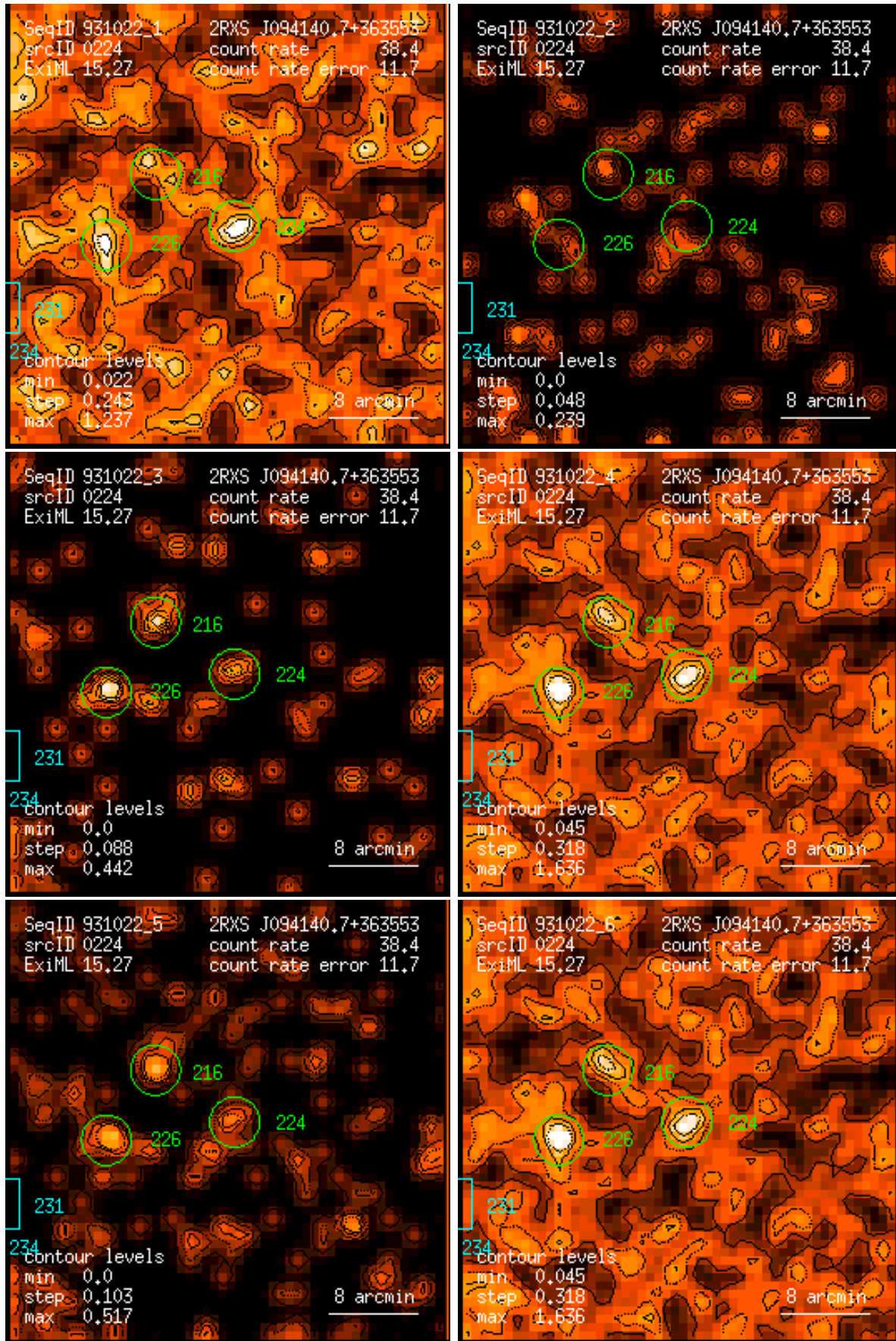
Figure 224: RASS 931022: detection 0224: band rate images, Gaussian filter: (1) PSPC channels 11 – 41, (2) 52 – 90, (3) 91 – 201, (4) 11 – 235, (5) 52 – 201, (6) 11 – 201. Broad band rates in counts/ks. Band rate contour levels in counts/ks/arcmin 2 .
