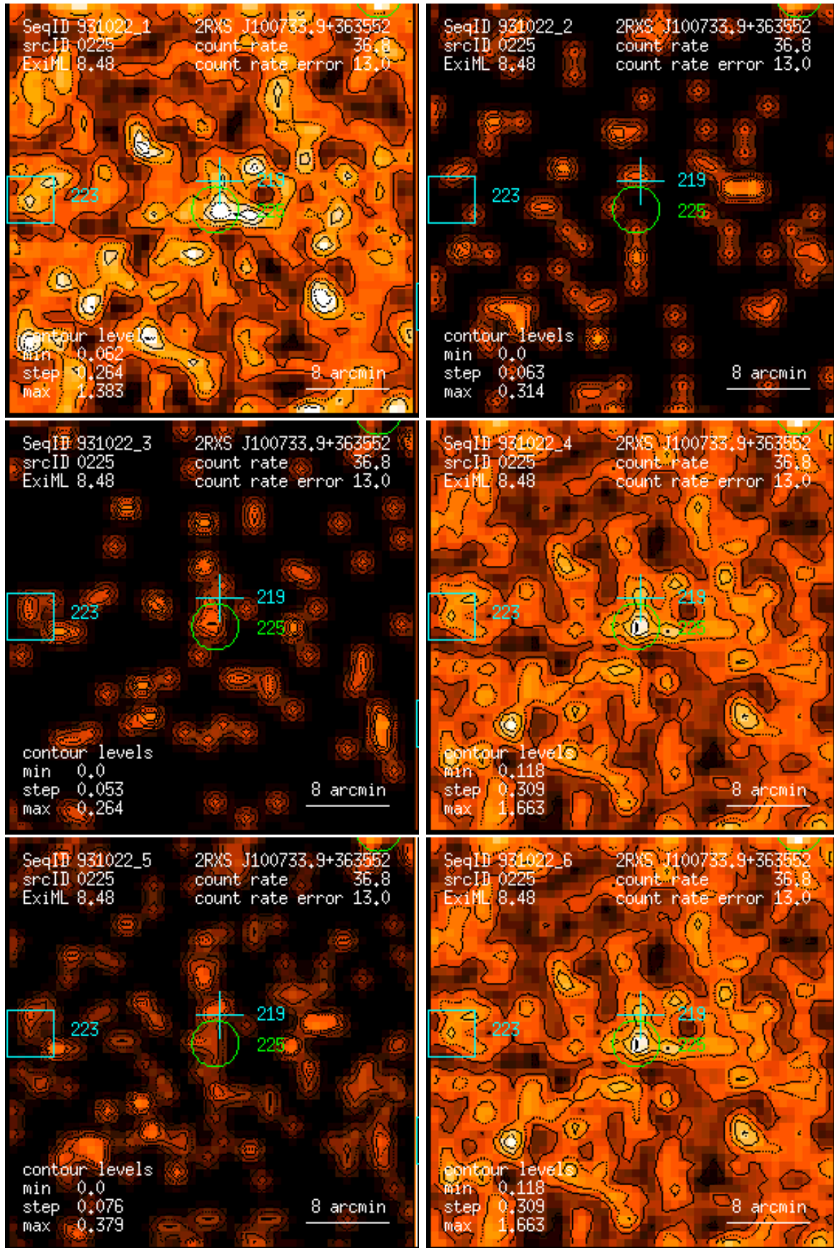
Figure 225: RASS 931022: detection 0225: band rate images, Gaussian filter: (1) PSPC channels 11 – 41, (2) 52 – 90, (3) 91 – 201, (4) 11 – 235, (5) 52 – 201, (6) 11 – 201. Broad band rates in counts/ks. Band rate contour levels in counts/ks/arcmin 2 .
