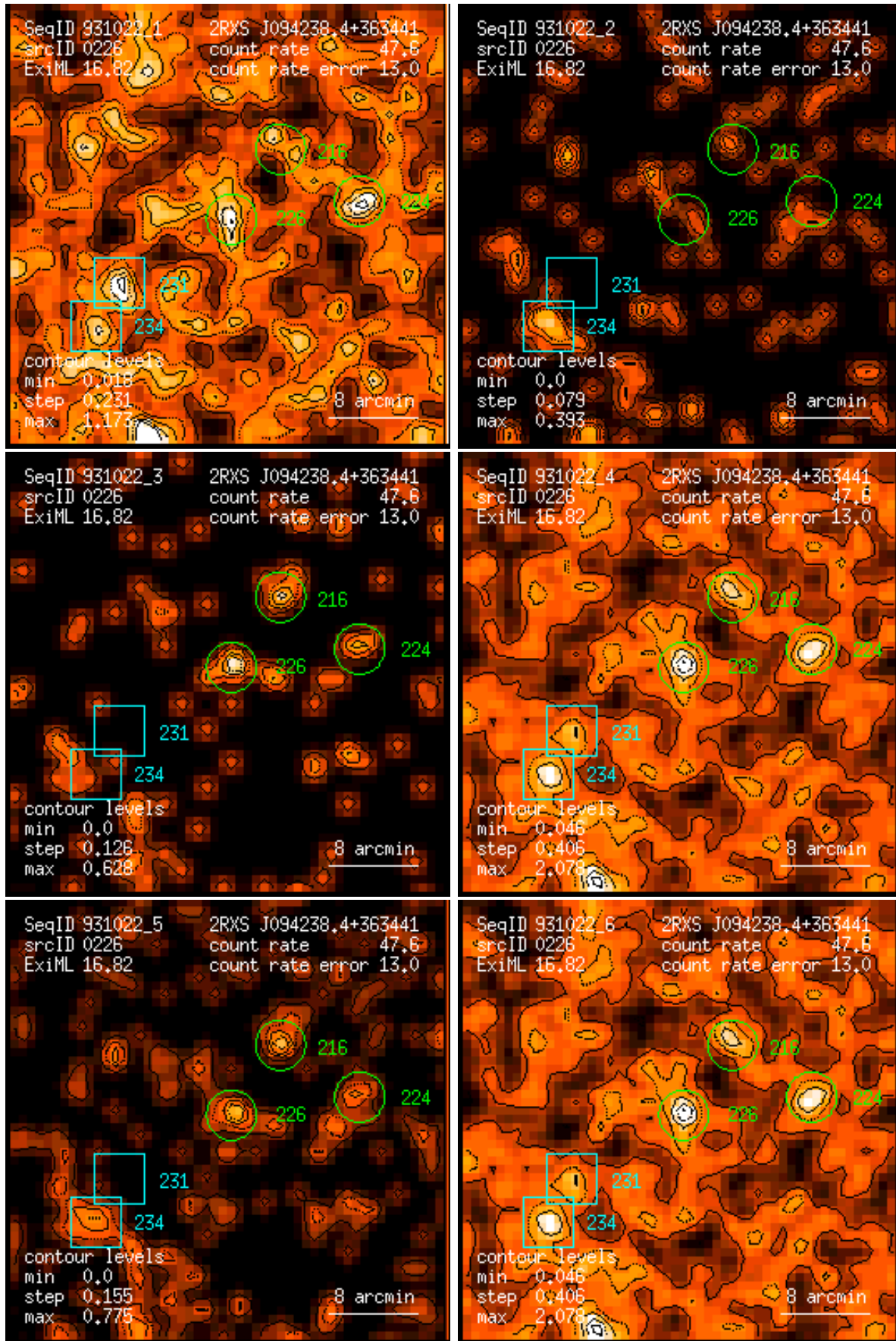
Figure 226: RASS 931022: detection 0226: band rate images, Gaussian filter: (1) PSPC channels 11 – 41, (2) 52 – 90, (3) 91 – 201, (4) 11 – 235, (5) 52 – 201, (6) 11 – 201. Broad band rates in counts/ks. Band rate contour levels in counts/ks/arcmin 2 .
