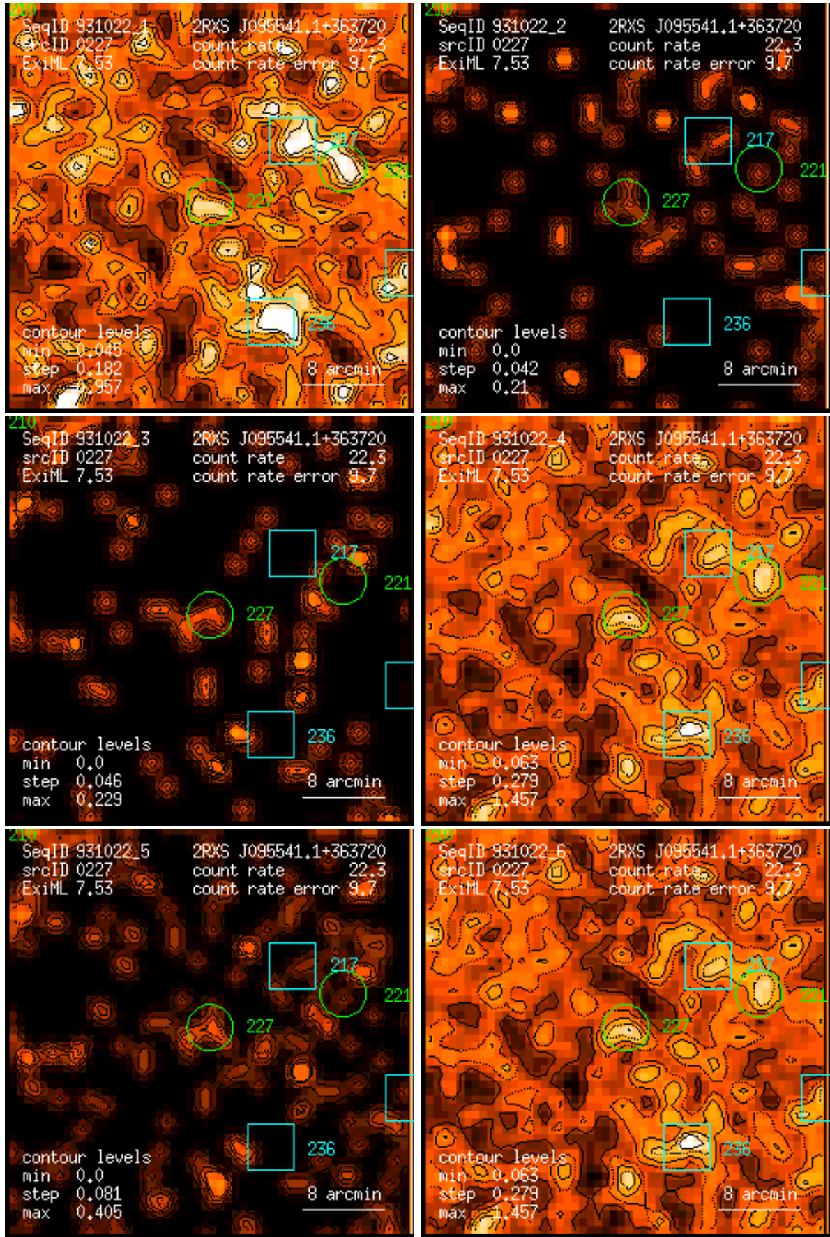
Figure 227: RASS 931022: detection 0227: band rate images, Gaussian filter: (1) PSPC channels 11 – 41, (2) 52 – 90, (3) 91 – 201, (4) 11 – 235, (5) 52 – 201, (6) 11 – 201. Broad band rates in counts/ks. Band rate contour levels in counts/ks/arcmin 2 .
