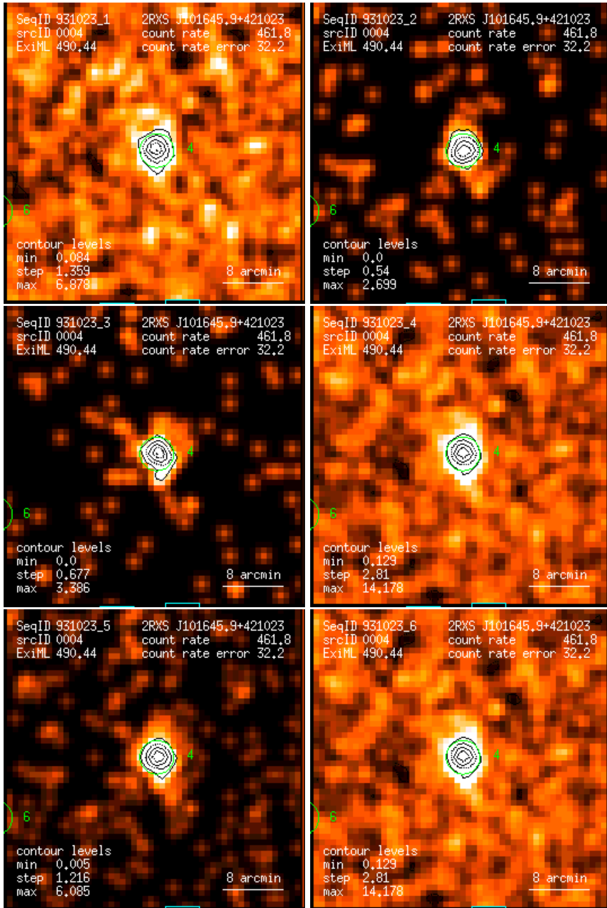
Figure 4: RASS 931023: detection 0004: band rate images, Gaussian filter: (1) PSPC channels 11 – 41, (2) 52 – 90, (3) 91 – 201, (4) 11 – 235, (5) 52 – 201, (6) 11 – 201. Broad band rates in counts/ks. Band rate contour levels in counts/ks/arcmin 2 .
