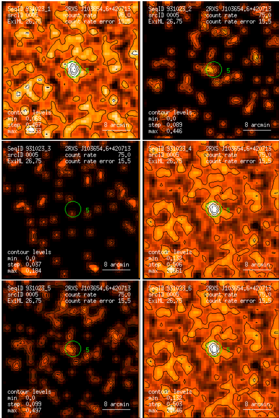
Figure 5: RASS 931023: detection 0005: band rate images, Gaussian filter: (1) PSPC channels 11 – 41, (2) 52 – 90, (3) 91 – 201, (4) 11 – 235, (5) 52 – 201, (6) 11 – 201. Broad band rates in counts/ks. Band rate contour levels in counts/ks/arcmin 2 .
