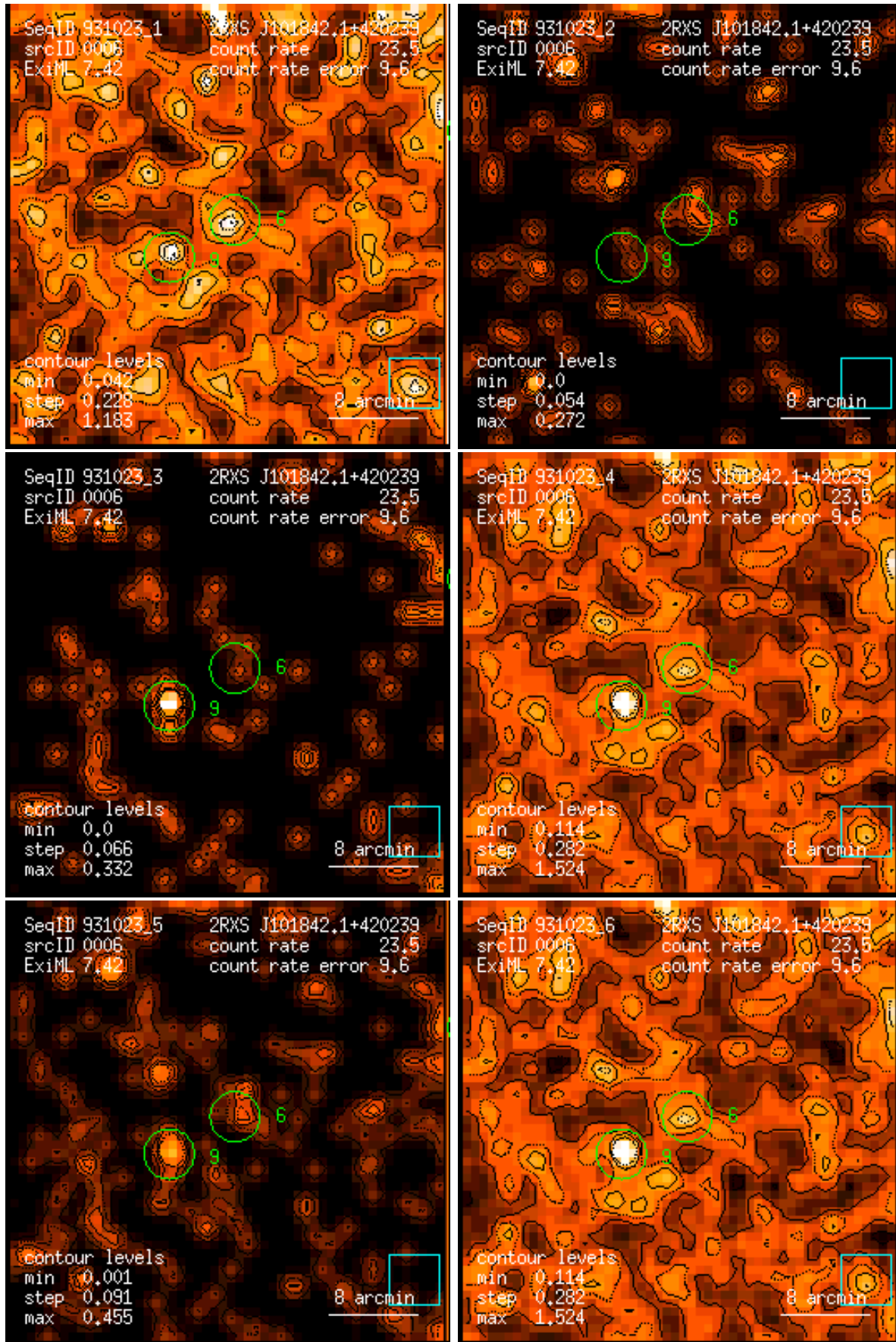
Figure 6: RASS 931023: detection 0006: band rate images, Gaussian filter: (1) PSPC channels 11 – 41, (2) 52 – 90, (3) 91 – 201, (4) 11 – 235, (5) 52 – 201, (6) 11 – 201. Broad band rates in counts/ks. Band rate contour levels in counts/ks/arcmin 2 .
