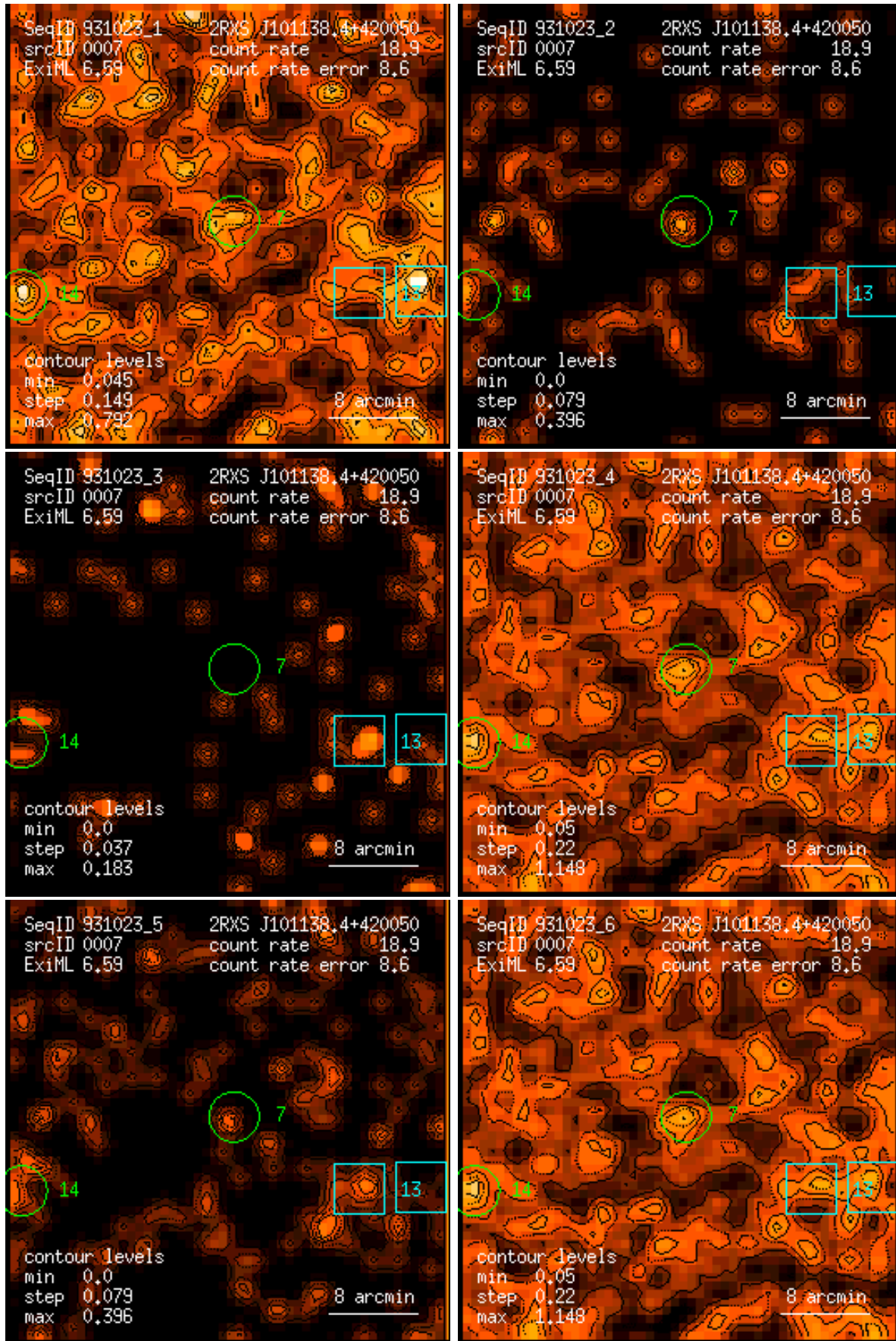
Figure 7: RASS 931023: detection 0007: band rate images, Gaussian filter: (1) PSPC channels 11 – 41, (2) 52 – 90, (3) 91 – 201, (4) 11 – 235, (5) 52 – 201, (6) 11 – 201. Broad band rates in counts/ks. Band rate contour levels in counts/ks/arcmin 2 .
