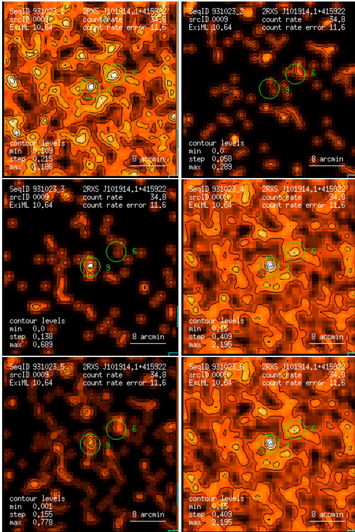
Figure 9: RASS 931023: detection 0009: band rate images, Gaussian filter: (1) PSPC channels 11 – 41, (2) 52 – 90, (3) 91 – 201, (4) 11 – 235, (5) 52 – 201, (6) 11 – 201. Broad band rates in counts/ks. Band rate contour levels in counts/ks/arcmin 2 .
