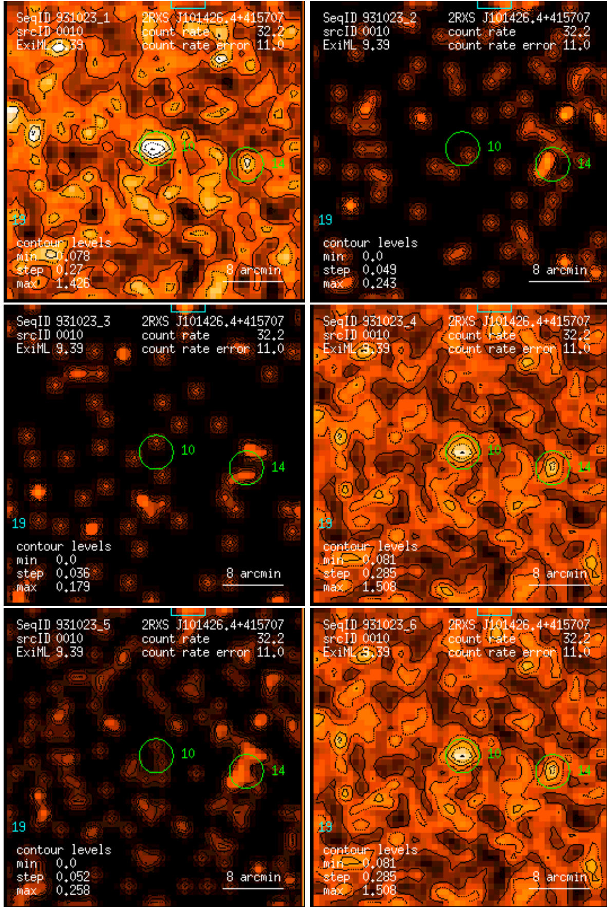
Figure 10: RASS 931023: detection 0010: band rate images, Gaussian filter: (1) PSPC channels 11 – 41, (2) 52 – 90, (3) 91 – 201, (4) 11 – 235, (5) 52 – 201, (6) 11 – 201. Broad band rates in counts/ks. Band rate contour levels in counts/ks/arcmin 2 .
