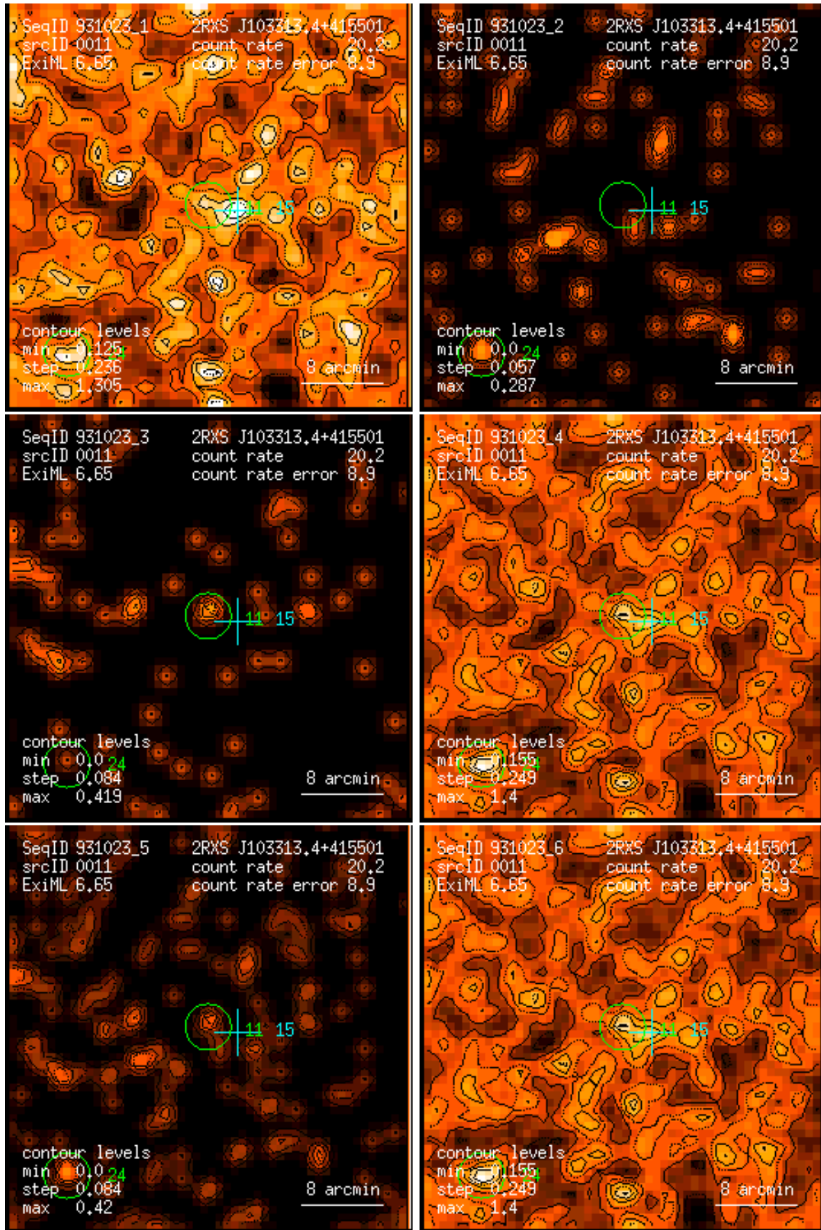
Figure 11: RASS 931023: detection 0011: band rate images, Gaussian filter: (1) PSPC channels 11 – 41, (2) 52 – 90, (3) 91 – 201, (4) 11 – 235, (5) 52 – 201, (6) 11 – 201. Broad band rates in counts/ks. Band rate contour levels in counts/ks/arcmin 2 .
