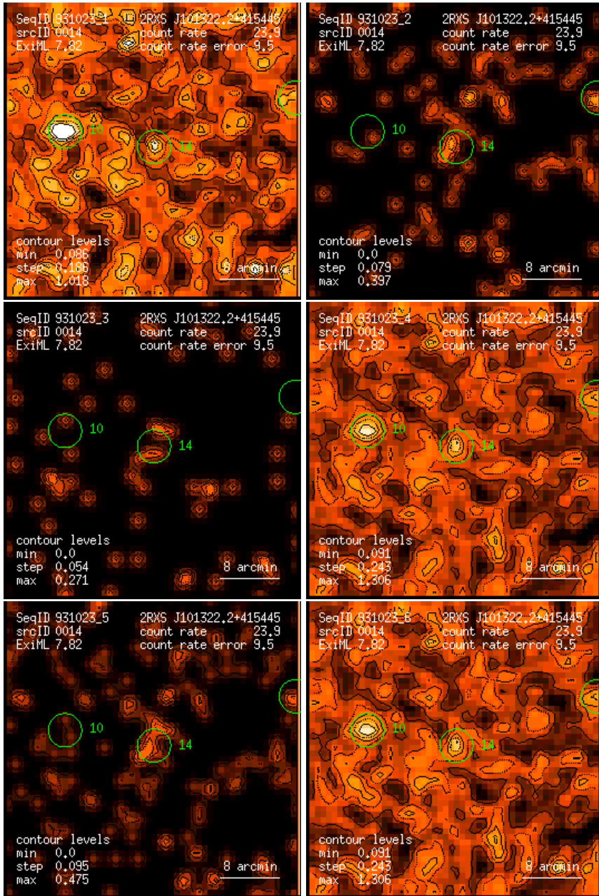
Figure 14: RASS 931023: detection 0014: band rate images, Gaussian filter: (1) PSPC channels 11 – 41, (2) 52 – 90, (3) 91 – 201, (4) 11 – 235, (5) 52 – 201, (6) 11 – 201. Broad band rates in counts/ks. Band rate contour levels in counts/ks/arcmin 2 .
