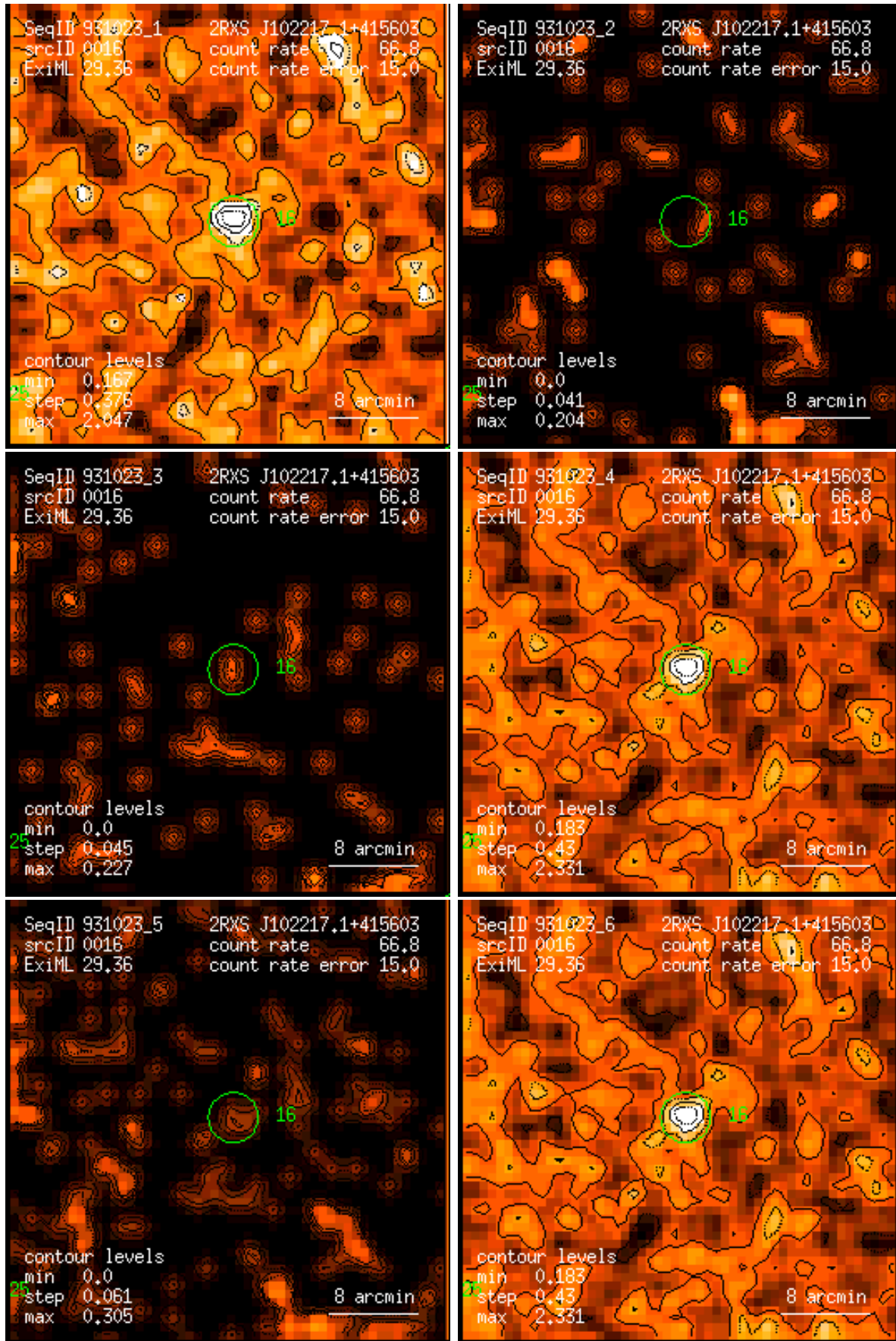
Figure 16: RASS 931023: detection 0016: band rate images, Gaussian filter: (1) PSPC channels 11 – 41, (2) 52 – 90, (3) 91 – 201, (4) 11 – 235, (5) 52 – 201, (6) 11 – 201. Broad band rates in counts/ks. Band rate contour levels in counts/ks/arcmin 2 .
