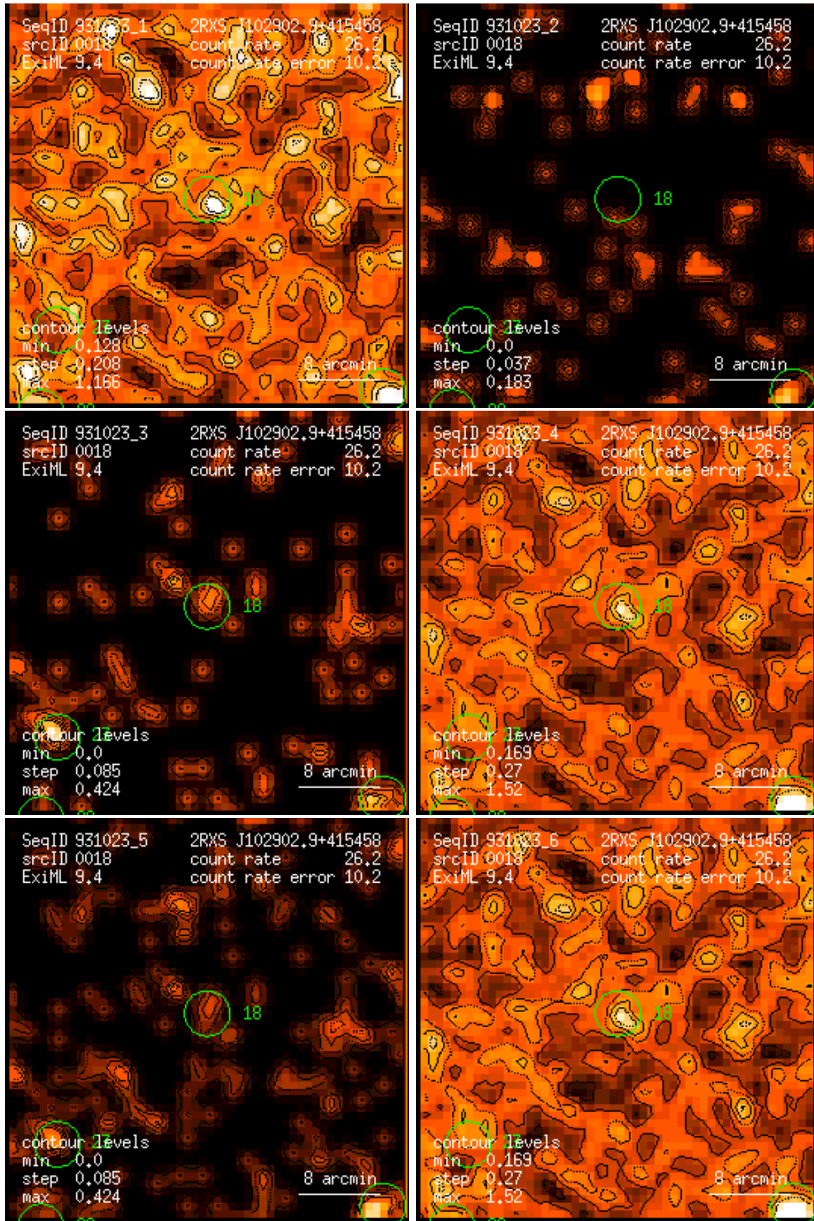
Figure 18: RASS 931023: detection 0018: band rate images, Gaussian filter: (1) PSPC channels 11 – 41, (2) 52 – 90, (3) 91 – 201, (4) 11 – 235, (5) 52 – 201, (6) 11 – 201. Broad band rates in counts/ks. Band rate contour levels in counts/ks/arcmin 2 .
