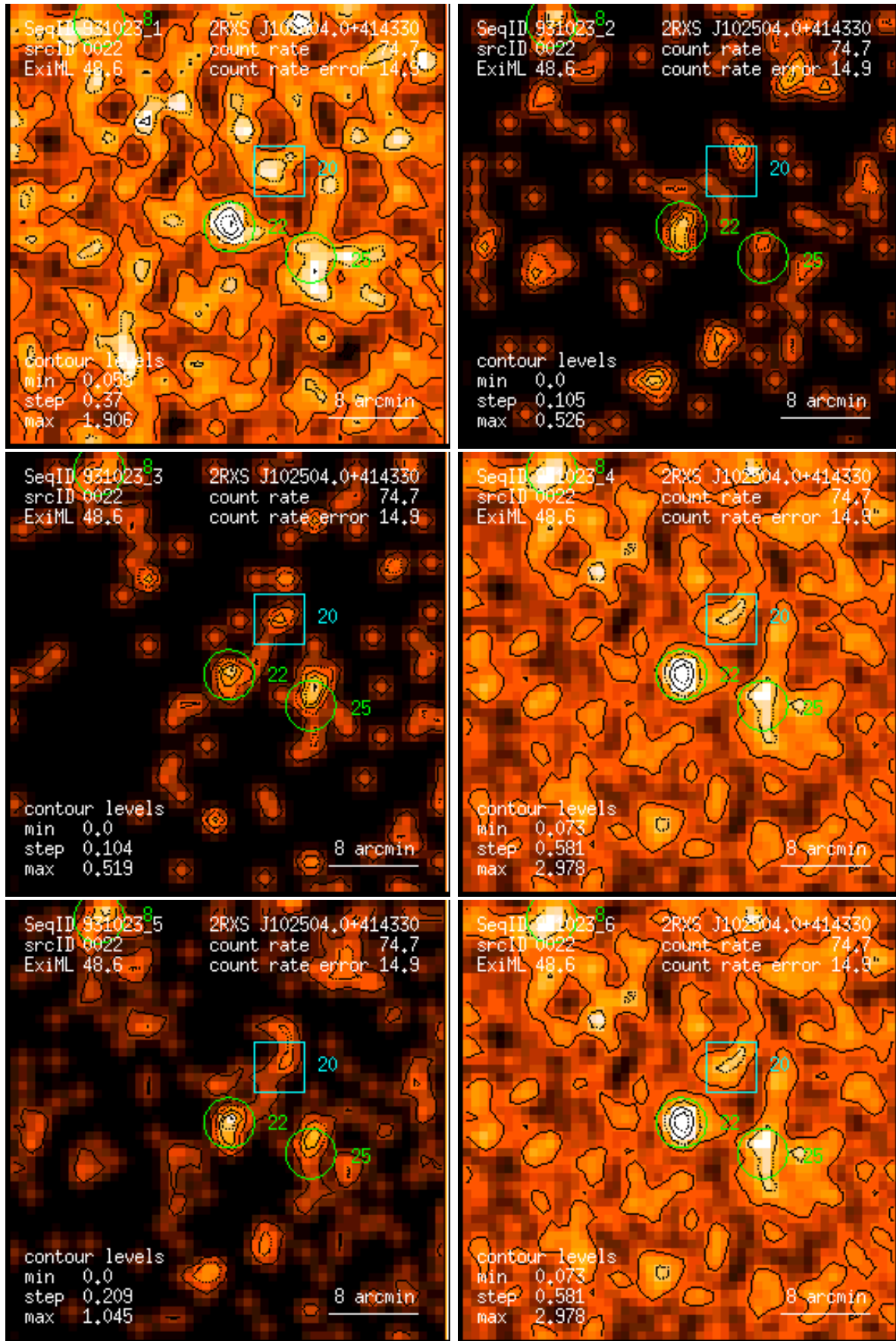
Figure 22: RASS 931023: detection 0022: band rate images, Gaussian filter: (1) PSPC channels 11 – 41, (2) 52 – 90, (3) 91 – 201, (4) 11 – 235, (5) 52 – 201, (6) 11 – 201. Broad band rates in counts/ks. Band rate contour levels in counts/ks/arcmin 2 .
