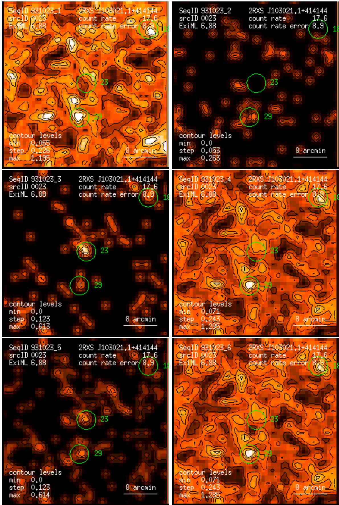
Figure 23: RASS 931023: detection 0023: band rate images, Gaussian filter: (1) PSPC channels 11 – 41, (2) 52 – 90, (3) 91 – 201, (4) 11 – 235, (5) 52 – 201, (6) 11 – 201. Broad band rates in counts/ks. Band rate contour levels in counts/ks/arcmin 2 .
