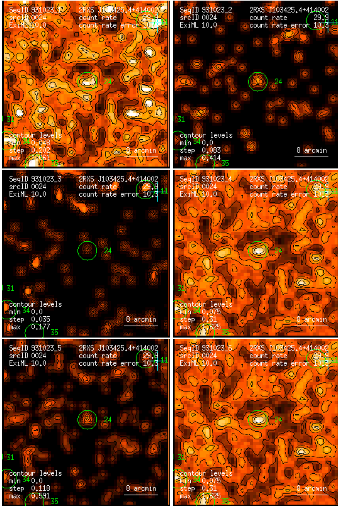
Figure 24: RASS 931023: detection 0024: band rate images, Gaussian filter: (1) PSPC channels 11 – 41, (2) 52 – 90, (3) 91 – 201, (4) 11 – 235, (5) 52 – 201, (6) 11 – 201. Broad band rates in counts/ks. Band rate contour levels in counts/ks/arcmin 2 .
