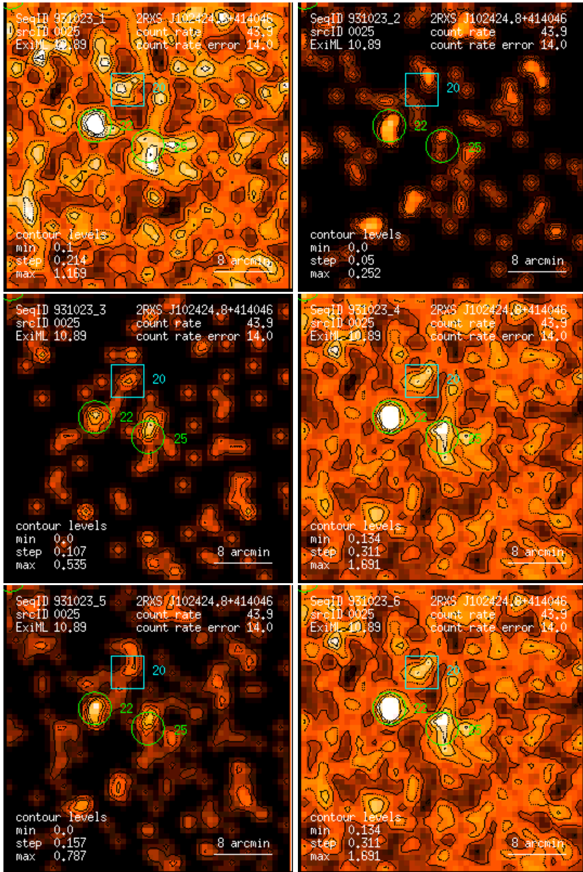
Figure 25: RASS 931023: detection 0025: band rate images, Gaussian filter: (1) PSPC channels 11 – 41, (2) 52 – 90, (3) 91 – 201, (4) 11 – 235, (5) 52 – 201, (6) 11 – 201. Broad band rates in counts/ks. Band rate contour levels in counts/ks/arcmin 2 .
