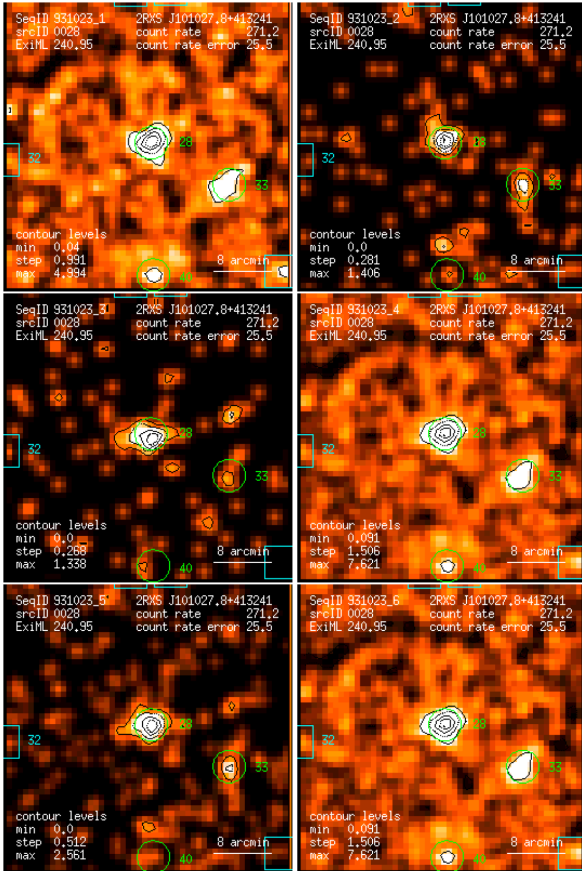
Figure 28: RASS 931023: detection 0028: band rate images, Gaussian filter: (1) PSPC channels 11 – 41, (2) 52 – 90, (3) 91 – 201, (4) 11 – 235, (5) 52 – 201, (6) 11 – 201. Broad band rates in counts/ks. Band rate contour levels in counts/ks/arcmin 2 .
