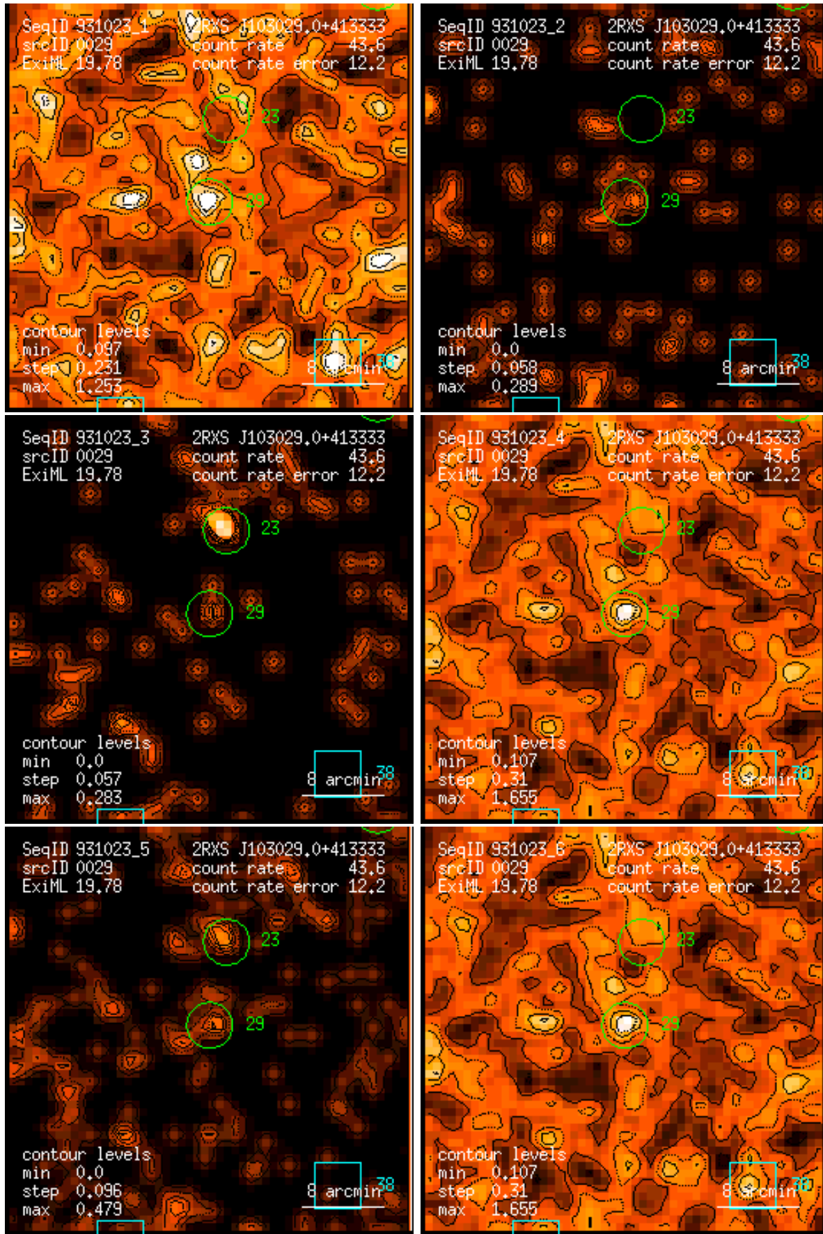
Figure 29: RASS 931023: detection 0029: band rate images, Gaussian filter: (1) PSPC channels 11 – 41, (2) 52 – 90, (3) 91 – 201, (4) 11 – 235, (5) 52 – 201, (6) 11 – 201. Broad band rates in counts/ks. Band rate contour levels in counts/ks/arcmin 2 .
