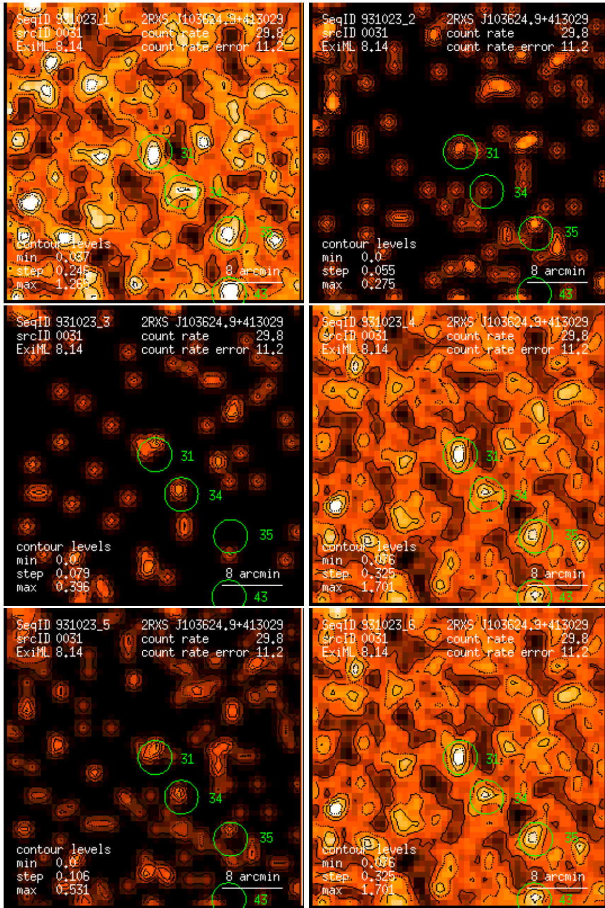
Figure 31: RASS 931023: detection 0031: band rate images, Gaussian filter: (1) PSPC channels 11 – 41, (2) 52 – 90, (3) 91 – 201, (4) 11 – 235, (5) 52 – 201, (6) 11 – 201. Broad band rates in counts/ks. Band rate contour levels in counts/ks/arcmin 2 .
