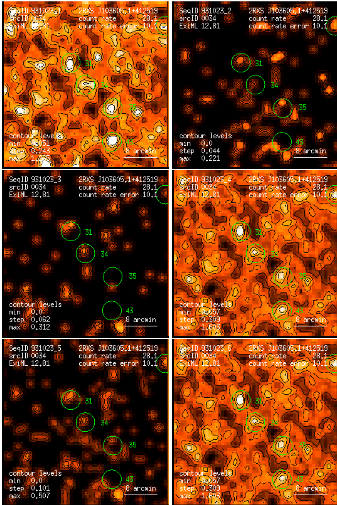
Figure 34: RASS 931023: detection 0034: band rate images, Gaussian filter: (1) PSPC channels 11 – 41, (2) 52 – 90, (3) 91 – 201, (4) 11 – 235, (5) 52 – 201, (6) 11 – 201. Broad band rates in counts/ks. Band rate contour levels in counts/ks/arcmin 2 .
