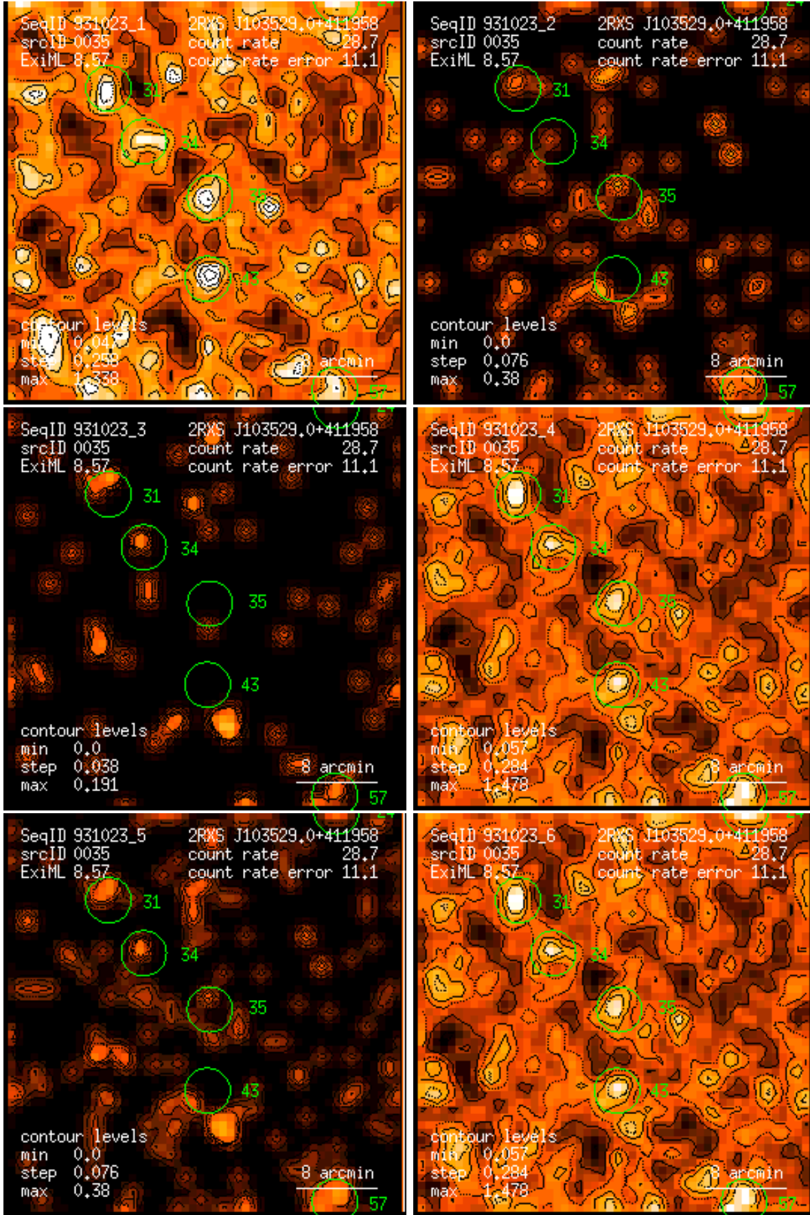
Figure 35: RASS 931023: detection 0035: band rate images, Gaussian filter: (1) PSPC channels 11 – 41, (2) 52 – 90, (3) 91 – 201, (4) 11 – 235, (5) 52 – 201, (6) 11 – 201. Broad band rates in counts/ks. Band rate contour levels in counts/ks/arcmin 2 .
