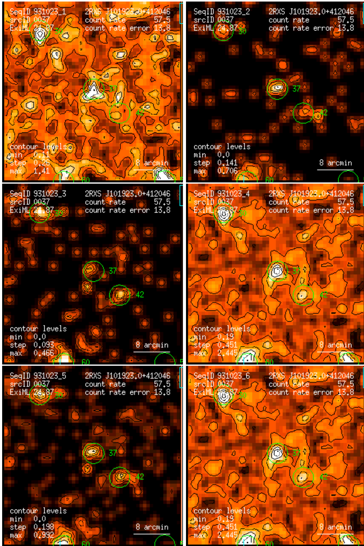
Figure 37: RASS 931023: detection 0037: band rate images, Gaussian filter: (1) PSPC channels 11 – 41, (2) 52 – 90, (3) 91 – 201, (4) 11 – 235, (5) 52 – 201, (6) 11 – 201. Broad band rates in counts/ks. Band rate contour levels in counts/ks/arcmin 2 .
